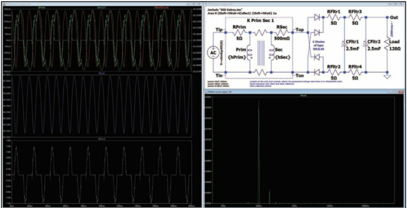
Figure 5c: The solution is not that obvious, but works like this: The resistors are split into four 5Ω resistors, and the capacitor is split into two 2.5mF capacitors, the same total values, 20Ω and 5mF but a completely different result.
