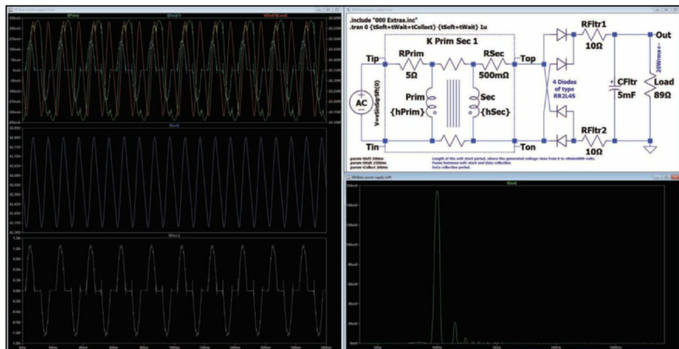
Figure 5b: In this variation, we chose some real filtering by adding RFitr1 and RFitr2, and keeping the 5mF capacitor.
