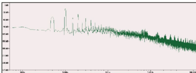
Photo 8: The FFT of the output wave shows a very slightly higher THD for the resistor version.
