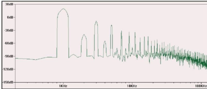
Figure 10: The FFT of the Class AB 2 output wave shows high upper-level harmonics.
