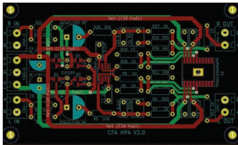
Figure 5: The main amp PCB layout was done with both a top and a bottom layer ground plane, along with power supply bypass caps adjacent to each of the IC power supply pins.
