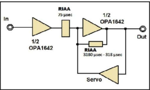
Figure 2: The detailed block diagram of the phono stage shows that each channel consists of two gain stages and a DC servo circuit that eliminates the output offset.
