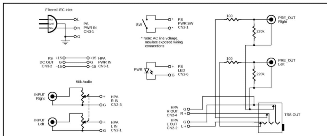
Figure 4: A switching headphone jack with connections to some RCA outputs with local loading resistors provide a separate preamp output.
