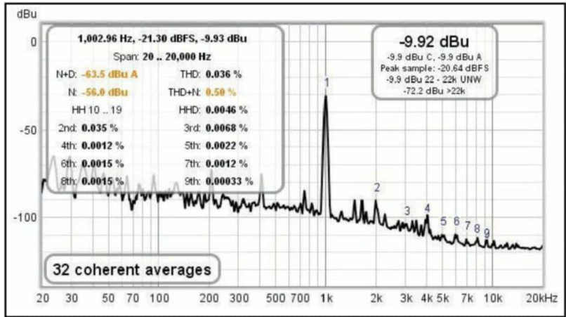
Figure 7: This graph shows the current feedback amplifier's THD measured at -10dBu output.
