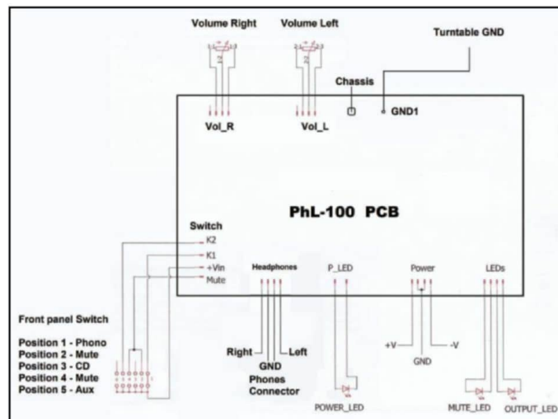
Figure 8: This diagram shows the internal wiring of the PhL-100.
