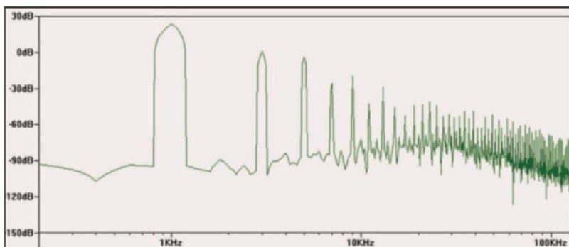
Figure 13: The FFT of the Class B amplifier clearly shows high levels of odd-order harmonics.
