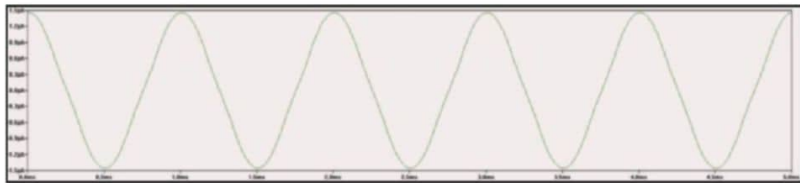
Figure 11: This control-grid current flows in the Class AB 2 circuit.
