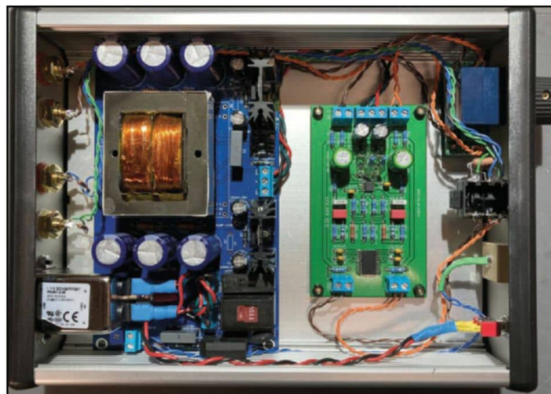
Photo 2: This top view photo includes the final version of the circuit board.
