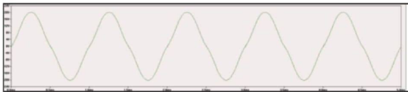
Figure 12: A true Class B amplifier would produce an output wave like this at a signal level near clipping.
