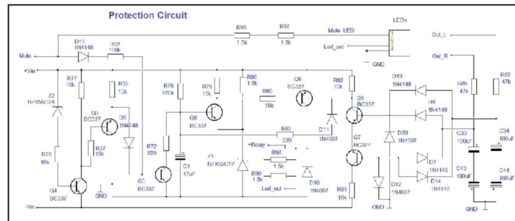
Figure 6: The protection circuit supports several functions.
