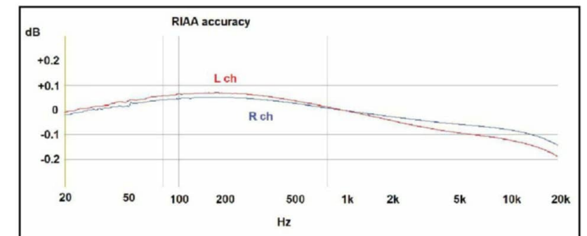
Figure 9: The accuracy of the RIAA response of the PhL-100 was tested.
