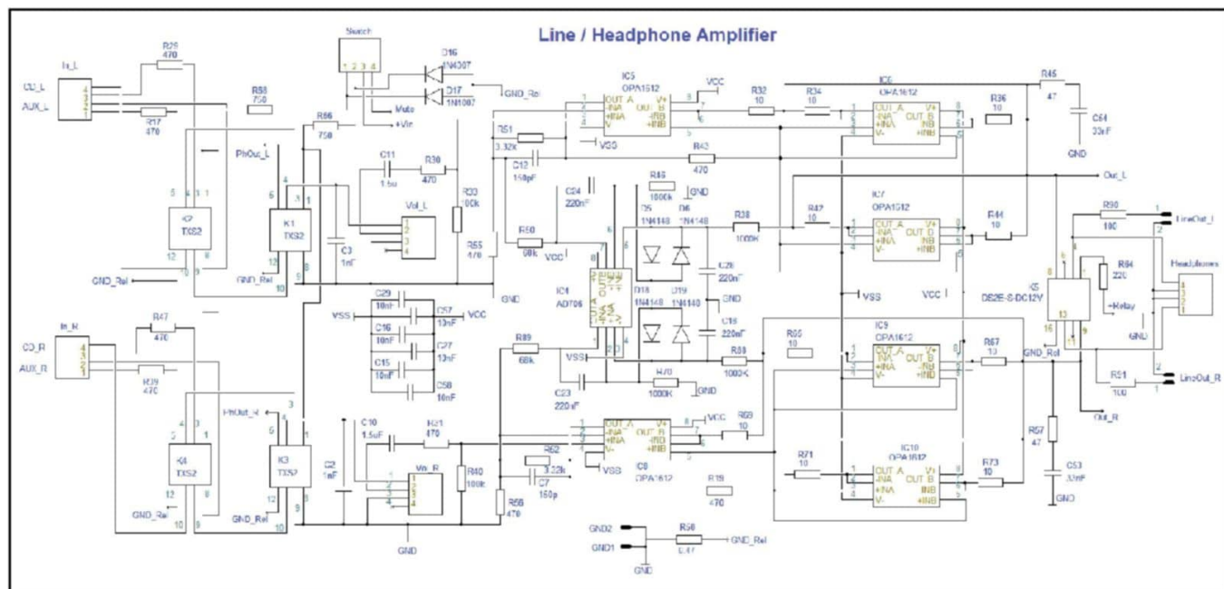
Figure 4: Here is the electronic schematic for the line and headphone amplifier.
