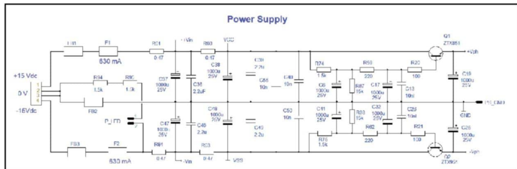
Figure 5: The schematic for the PhL-100's power supply circuit is shown here.
