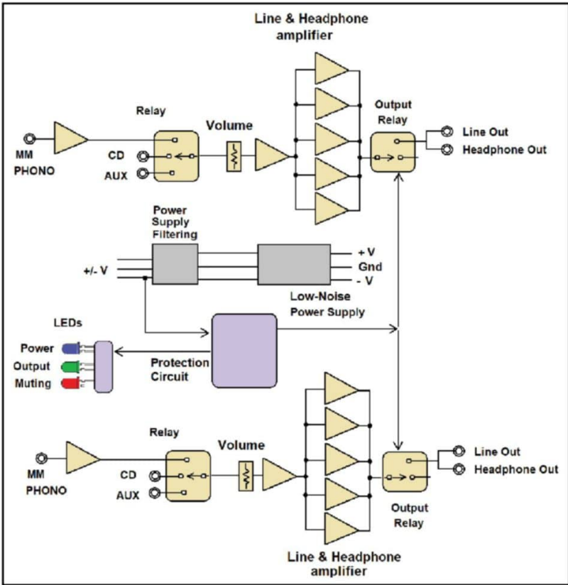
Figure 1: The simplified block diagram shows all the parts of the PhL-100 device, including a protection circuit.
