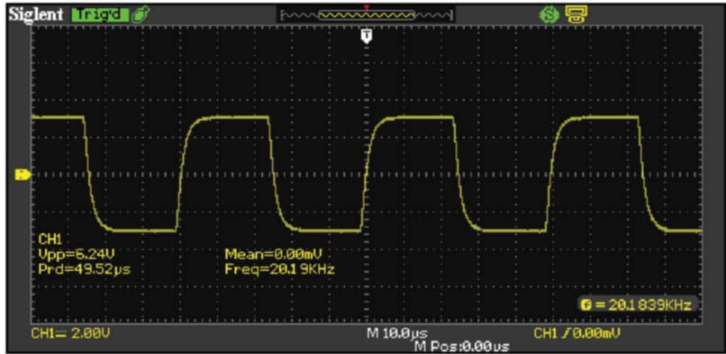
Figure 6: This test measurement shows the current feedback amplifier at 20kHz at 1W output into 39Ω
