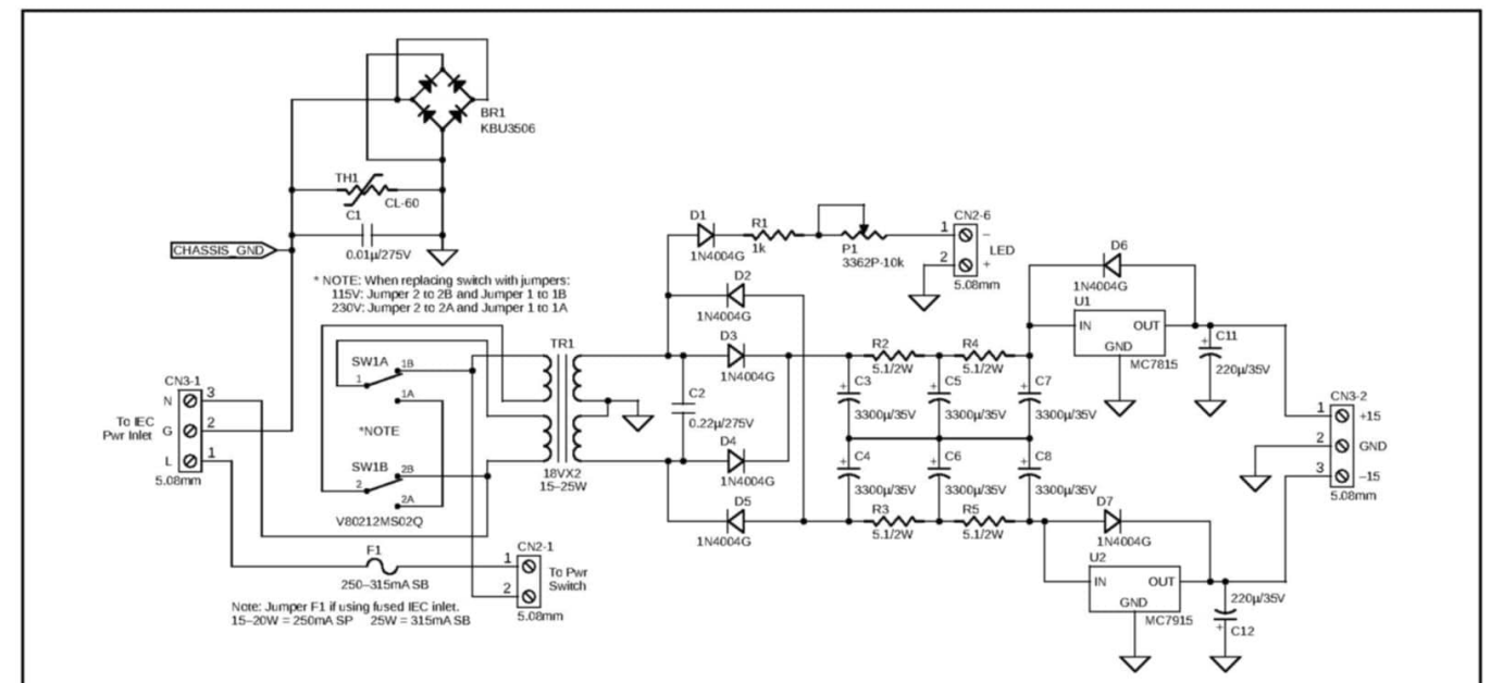
Figure 3: For the power supply, I used a 20W, \pm 15\text{VDC} regulated linear supply.
