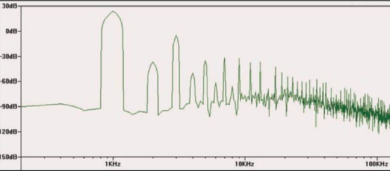
Figure 8: The FFT of the Class AB 1 output wave shows an increase in higher-order harmonics, compred to that of the Class A amplifier.
