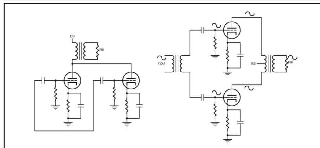
Figure 2: Class A amplifiers may be made to produce higher output powers by the use of parallel or push-pull topologies.
