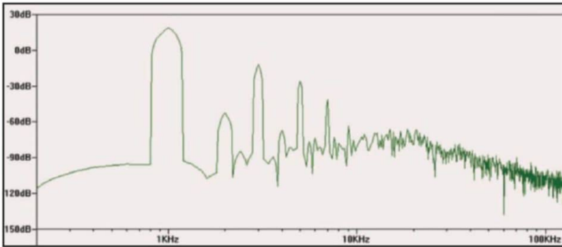
Figure 6: The FFT of the Class A output wave shows a preponderance of odd harmonics.
