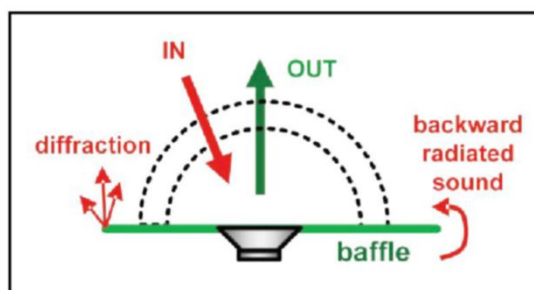
Figure 3: Direct sound separation for half-space measurement.
