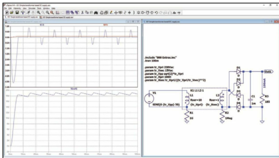
Figure 1: A simple transformer-based DC supply
