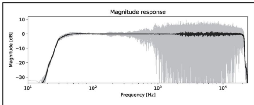
Figure 3: The measured response of a system using loudspeaker co-optimization for room correction, reflecting a flattening out, a reduction in spatial variations, and cancellation of room resonances.
