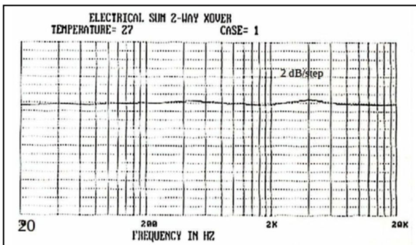
Figure 6: Here is the crossover electrical sum from the model. Note how closely the response here matches the acoustic measurements shown in Figure 2.
