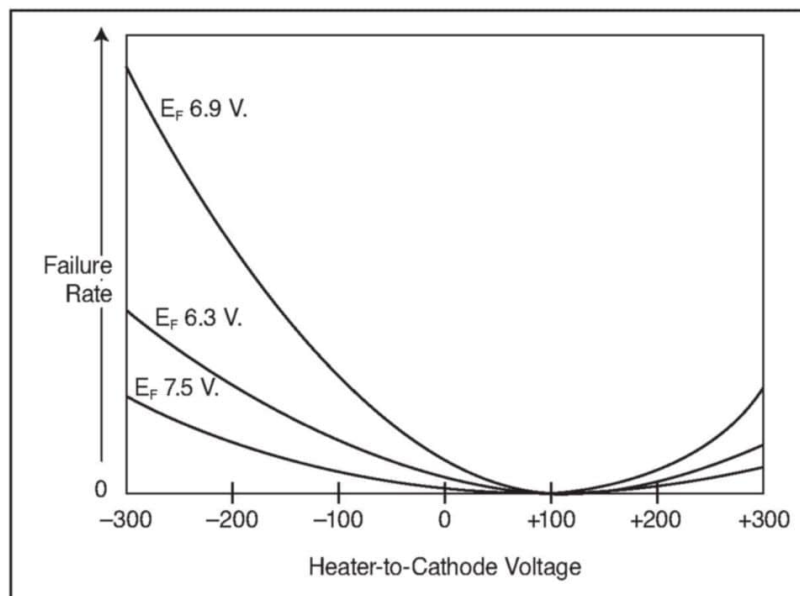
Figure 3: Increasing V_{kf} above approximately 90 V decreases tube lifetime.
