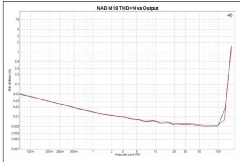
Figure 2: This plot of THD+N as a function of power shows the M10's nCore amps comfortably exceeding specifications.
