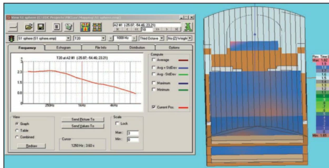
Figure 2: This graph shows RT vs. frequency and a map of RT in various positions in an auditorium. An omni speaker was used.
