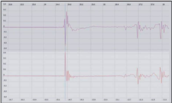
Figure 6: Comparing the ungated in-room impulse response of the left speaker uncorrected (upper) and the same impulse with Dirac Live correction (lower) shows a remarkable improvement in phase coherence over the first few milliseconds.
