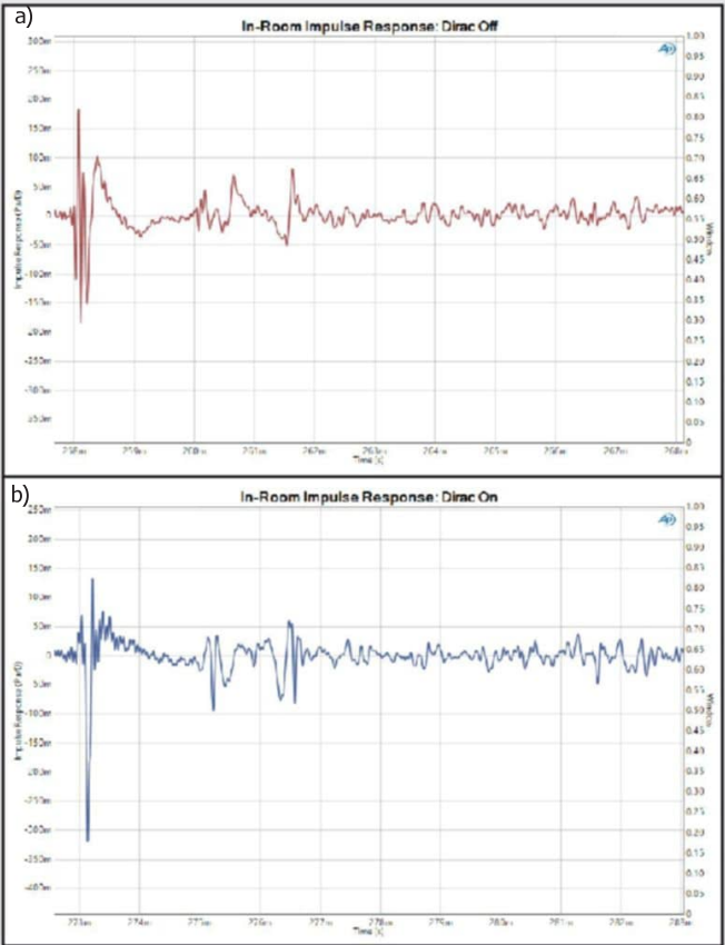
Figure 9: The impulse response of a mono signal driving both speakers taken at the listening position shows a marked increase in coherence when comparing uncorrected (a) with corrected by Dirac (b).
