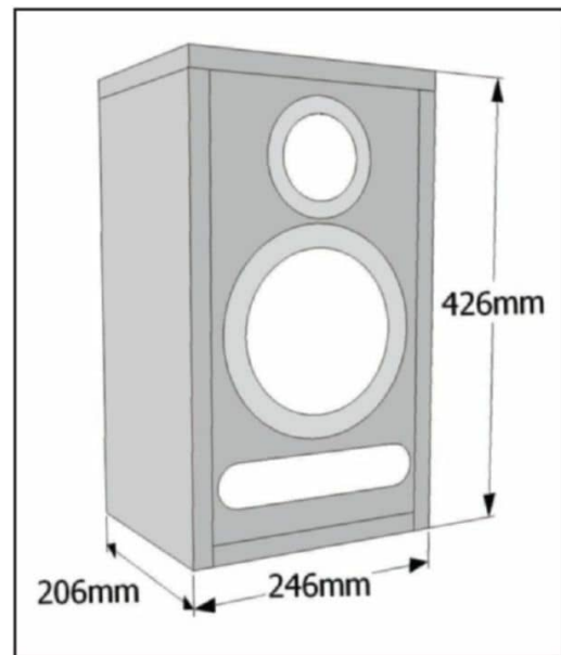
Figure 6: I used these dimensions to build the APR-17 loudspeaker.
