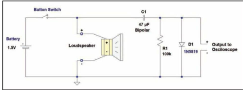
Figure 2: I used this circuit for the damping measurement.
