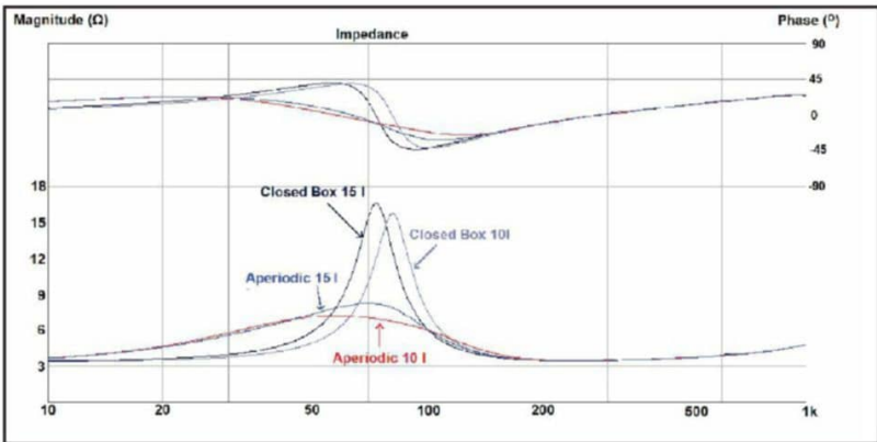
Figure 4: I took these woofer impedance measurements for the closed and the aperiodic test box.
