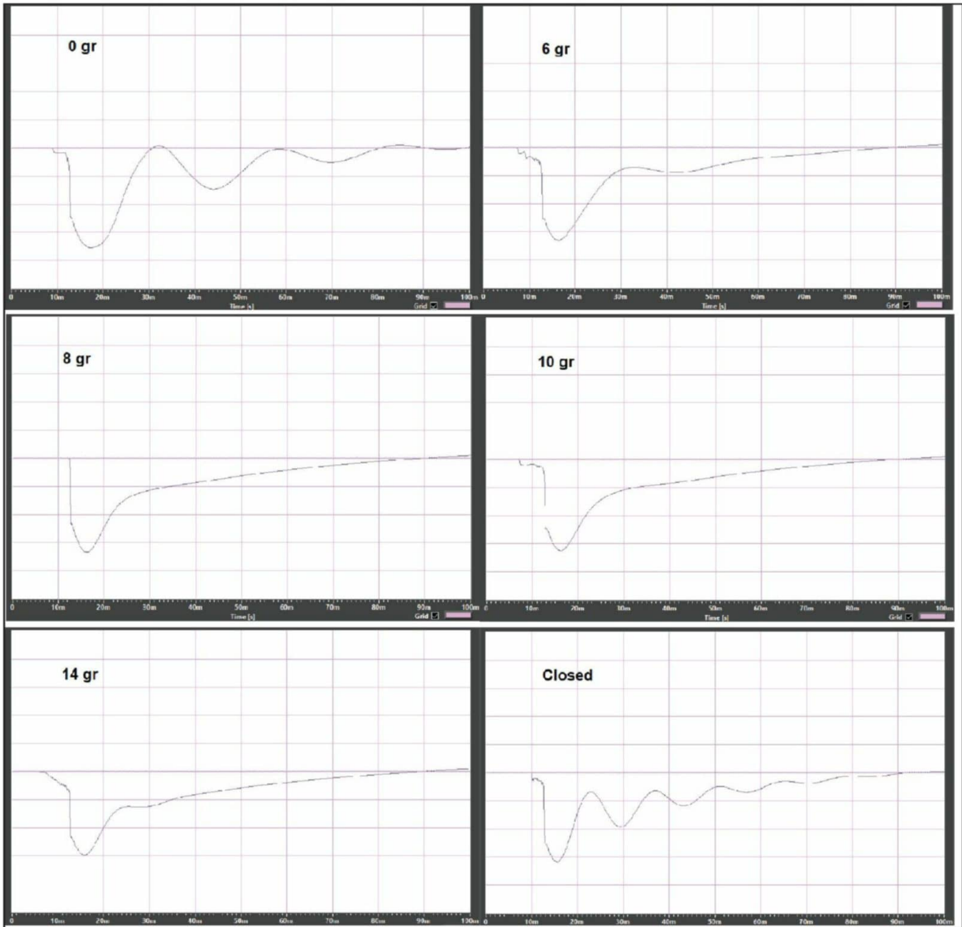
Figure 3: These are the oscilloscope traces of the woofer voltage with different aperiodic vent damping.
