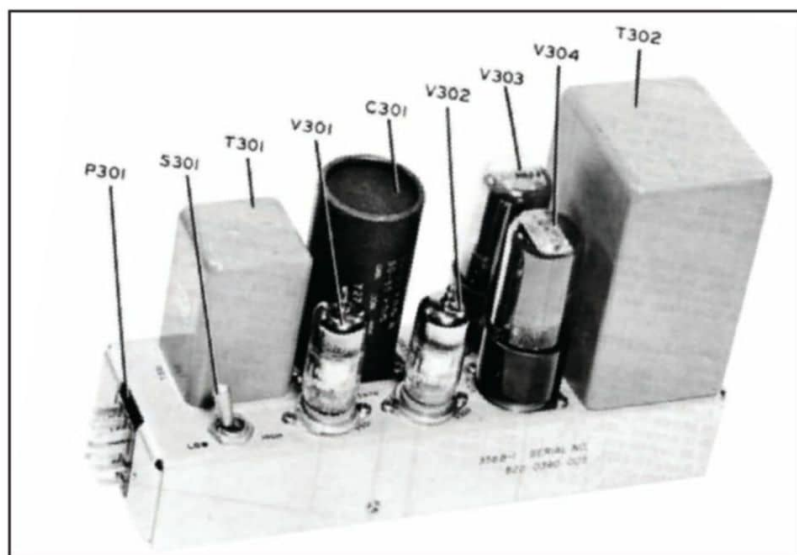
Photo 9: The Collins model 356B-1 main/program amplifier used in the 212 mixer was also modular.
