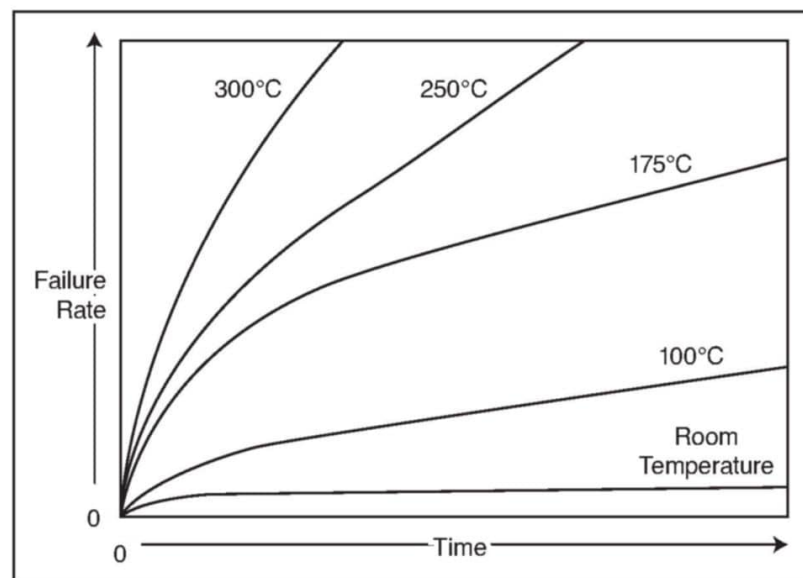
Figure 2: Insufficient air circulation heats up the tube envelope and drastically decreases tube lifetime.
