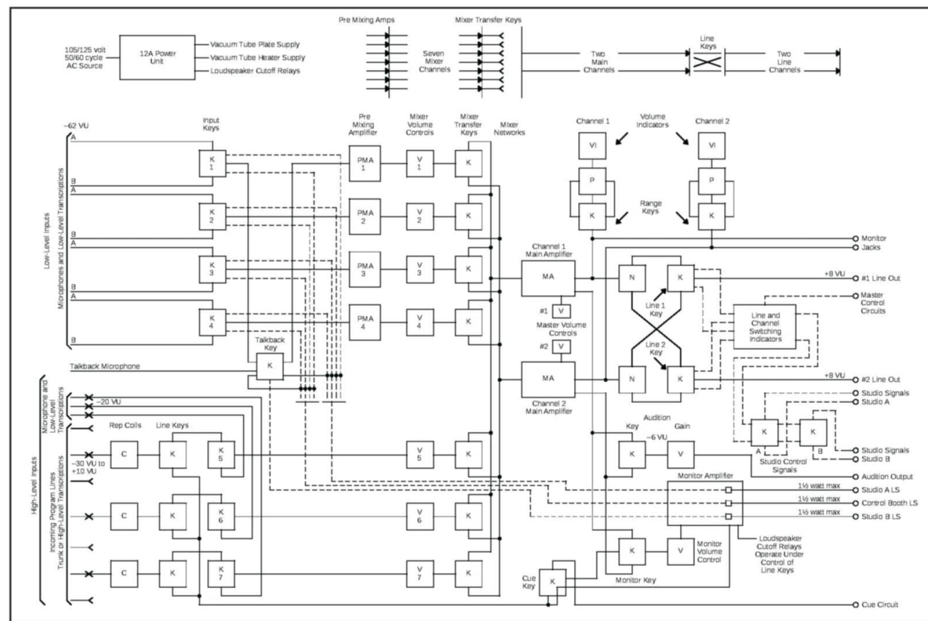
Figure 1: This functional block diagram of the WE 25B mixer is similar to that of most mixers of its era.
