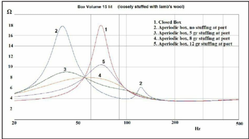
Figure 1: Impedance measurements for the 15 ltr test enclosure
