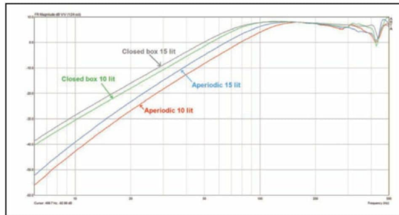
Figure 5: These are the frequency responses measurements for the closed and the aperiodic test box.
