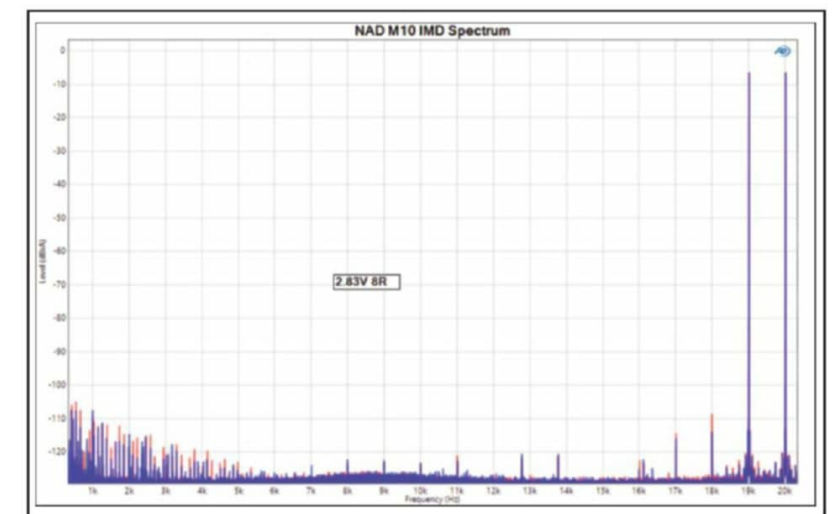
Figure 4: The 19+20kHz intermodulation spectrum of the M10 is extremely clean.
