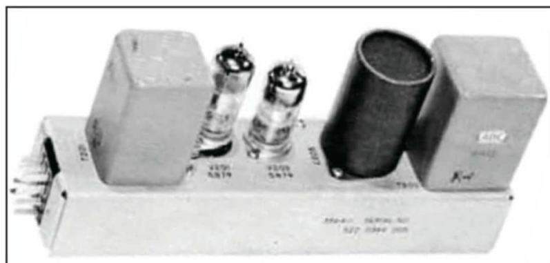
Photo 8: This two-stage plug-in preamplifier allowed easy servicing.
