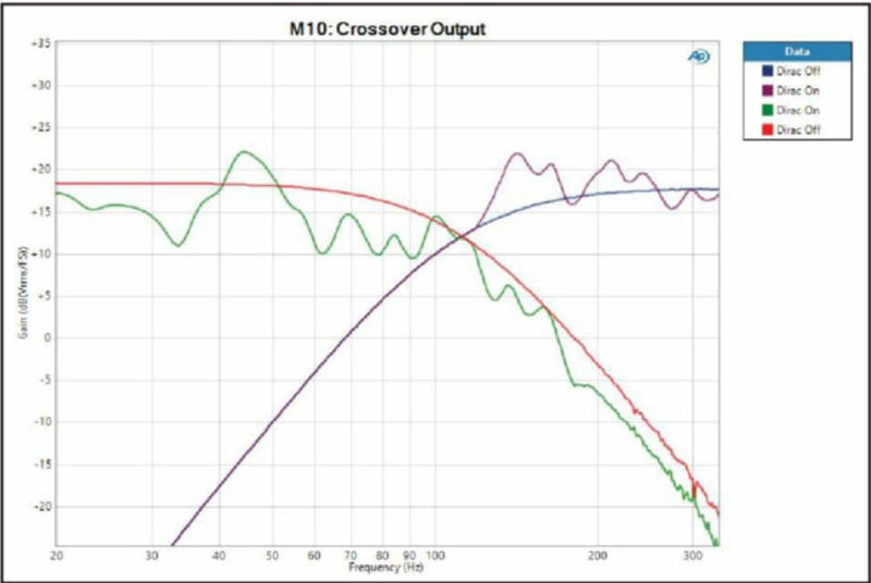
Figure 6: The subwoofer crossover of the M10 provides 24 dB/octave Linkwitz-Reilly filtering. The electrical output with Dirac Live turned on shows the applied correction response.
