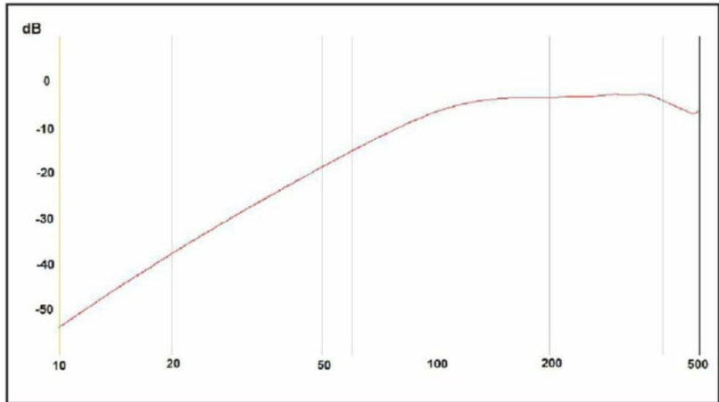
Figure 8: Here is the low-frequency response of the APR-17 woofer without crossover.
