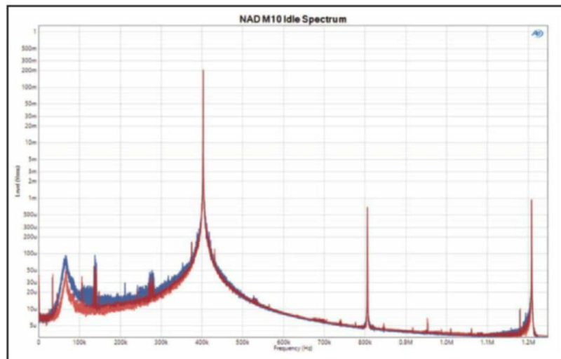
Figure 5: The M10's wideband (up to 1.2 MHz) noise spectrum indicates very low levels of ultrasonic and switching noise.
