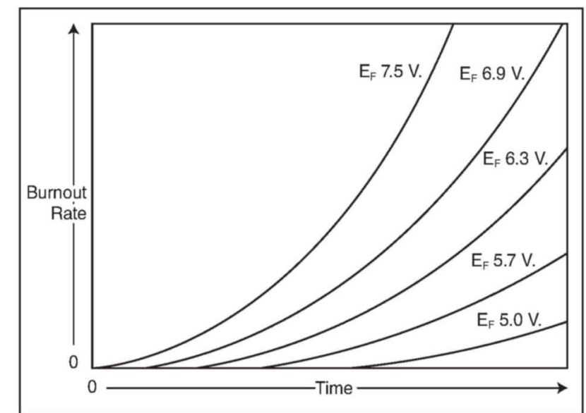
Figure 1: Increased heater voltage over the design value decreases tube lifetime.
