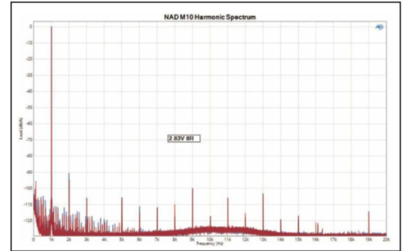
Figure 3: The harmonic distortion spectrum of the M10 at low power is dominated by small amounts of low-order distortion.
