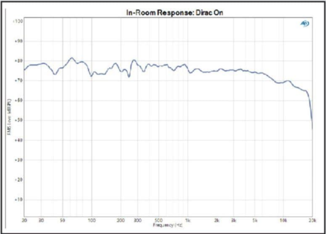
Figure 8: Taking the same measurement as in Figure 7, but with Dirac Live switched on, shows a significant improvement in the flatness of the response.
