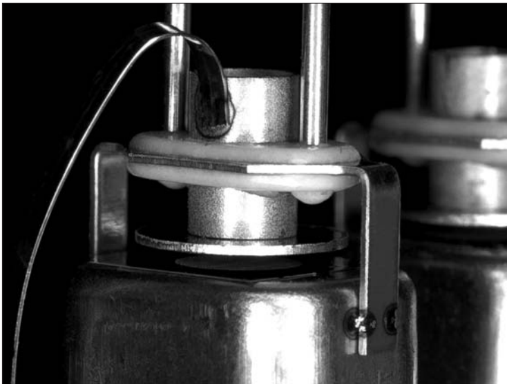
PHOTO 6: Close-up of grid assembly.
