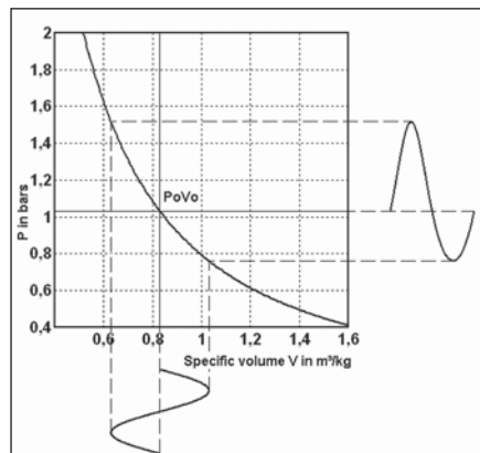
FIGURE 40: Adiabatic curve for air.
