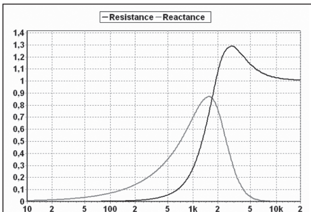
FIGURE 27: Normalized throat impedance of a 60° included angle infinite oblate spheroidal waveguide.
