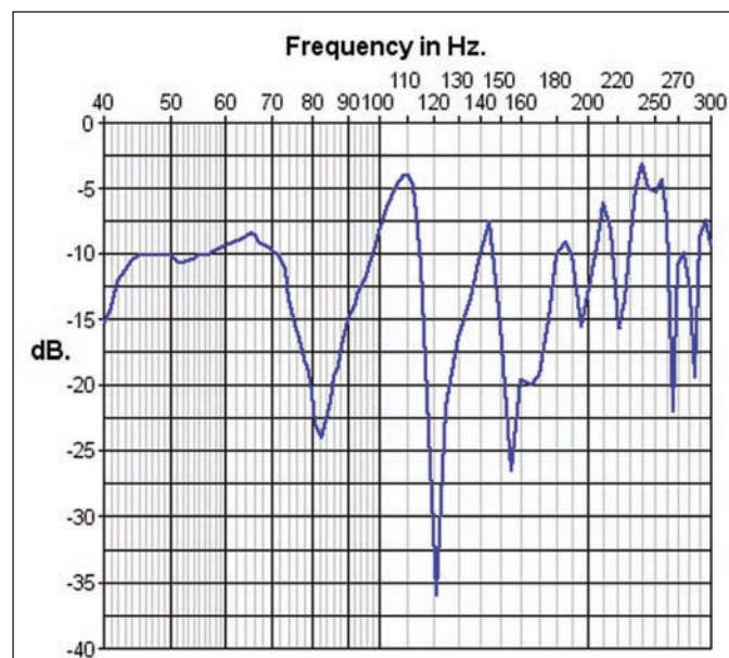
FIGURE 1: This frequency response was measured in a typical untreated listening room 16' long by 10' wide.
