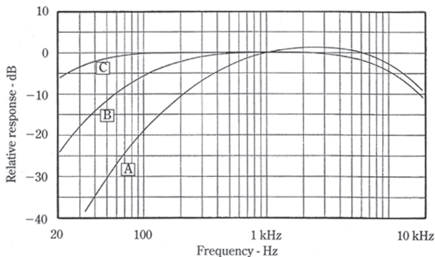
FIGURE 3: A, B, and C weighting response characteristics for sound level meters. [F. Alton Everest, Master Handbook of Acoustics (McGraw-Hill, New York, 2001), pp. 39, Fig. 2-31].
