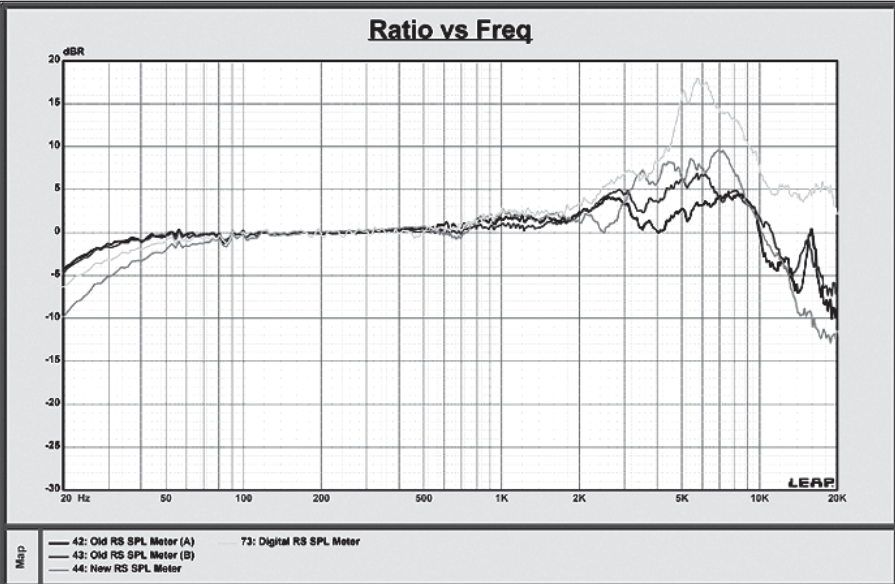
FIGURE 2: Calculated RS SPL meter frequency responses, relative to calibrated Mitey Mike II and associated electronics.
