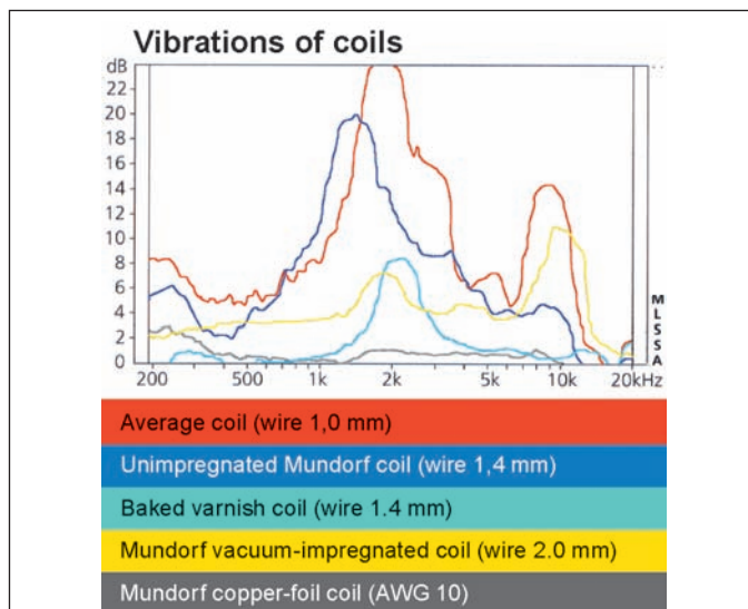
FIGURE 1: Vibration of coils of various constructions with signal frequency.
