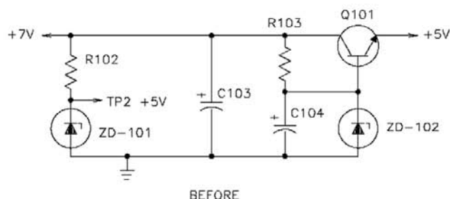
FIGURE 1: IG-4505 5V power supply redesign.
