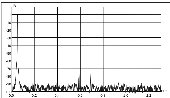
FIGURE 6: Spectrum of 50Hz sine wave (OPA604).
