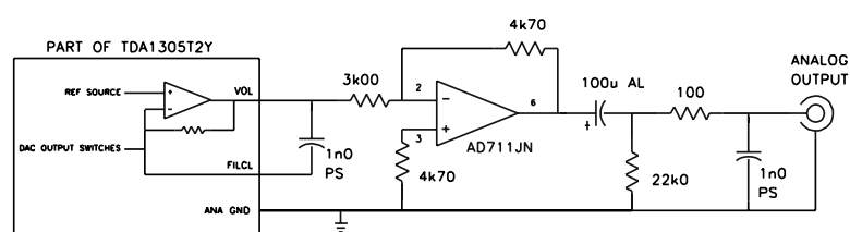
FIGURE 1: RCD 970BX analog output stage.
