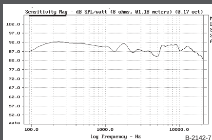
FIGURE 7: Average horizontal response \pm 30^\circ .
