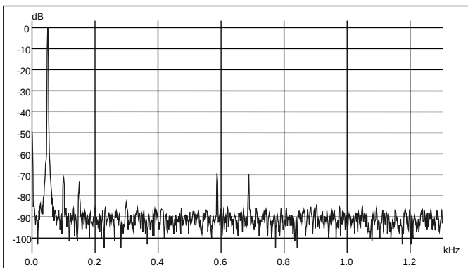
FIGURE 5: Spectrum of 50Hz sine wave (AD711).
