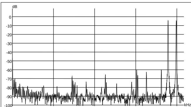
FIGURE 7: Intermodulation distortion, 19 + 20kHz 0dBfs (AD711).
