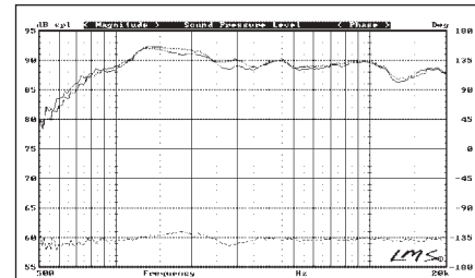
FIGURE 21: SPL of tweeter on enclosure with 1" beveled shell versus enclosure without edge treatment (solid line); difference curve raised 60dB.
