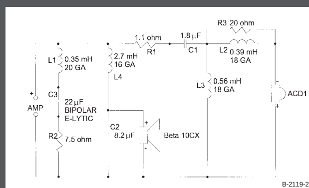
FIGURE 2: Crossover schematic (from Adire Audio assembly instructions).
