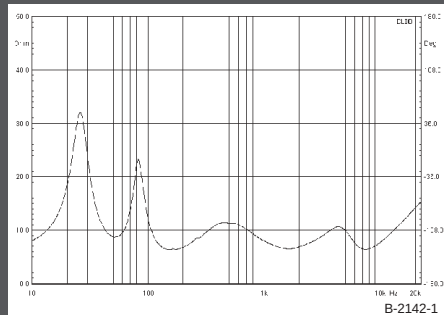
FIGURE 1: Adire impedance plot.
