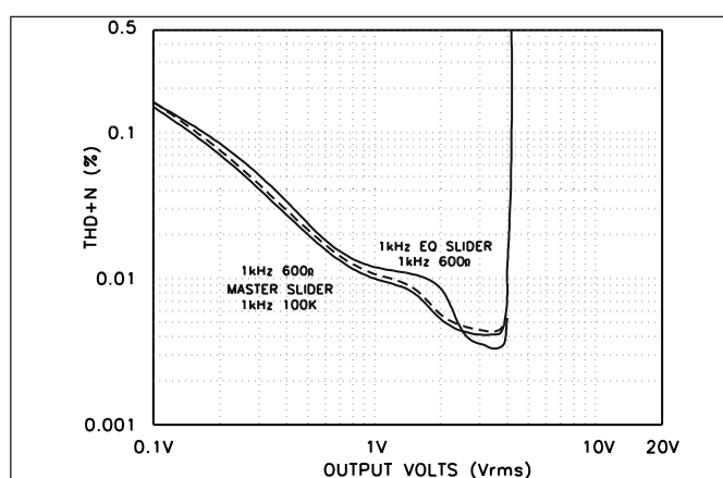
FIGURE 4: THD+N versus output.
