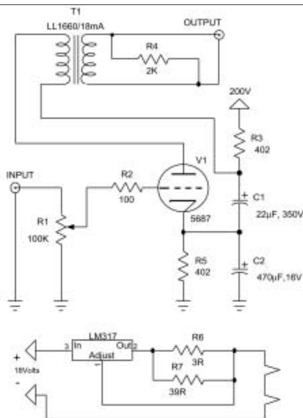
FIGURE 5: Single-ended line stage. This very good traditional transformer-output line stage came as a result of testing several options.
