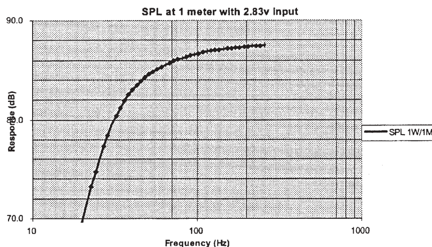
FIGURE 6: Bacon's proposed alignment for vented boxes, which allows for better transient response and is more forgiving of environment. Driver Q_{TS} = 0.3 , f_s = 30 , V_{AS} = 50 ltr.
