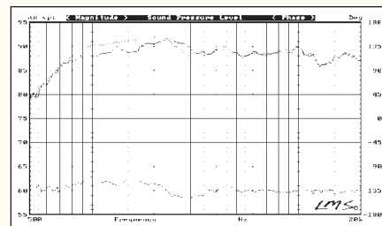
FIGURE 3: SPL of tweeter on IEC baffle with midbass uncovered (solid line) versus enclosure in free air; difference curve shows diffraction from enclosure edges.
