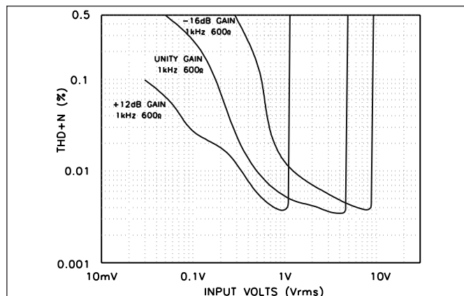
FIGURE 3: THD+N versus input.
