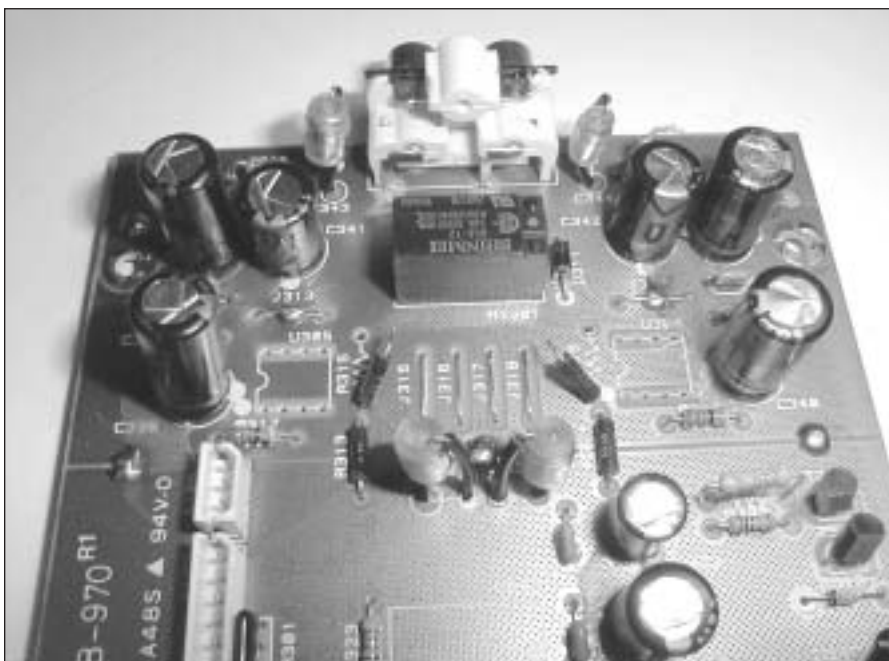
PHOTO 3: Board with ICs removed and resistors lifted.
