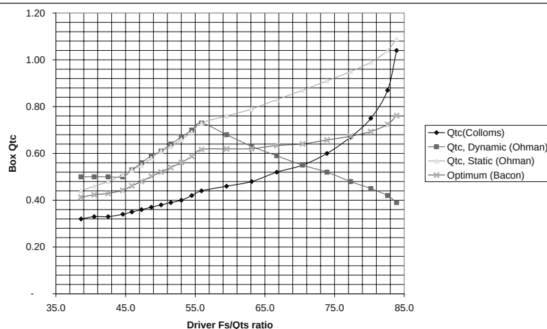
FIGURE 1: Best closed-box Q_{TC} as a function of driver f_s/Q_{TS} ratios.
