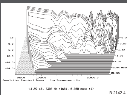
FIGURE 4: Adire cumulative spectral decay.
