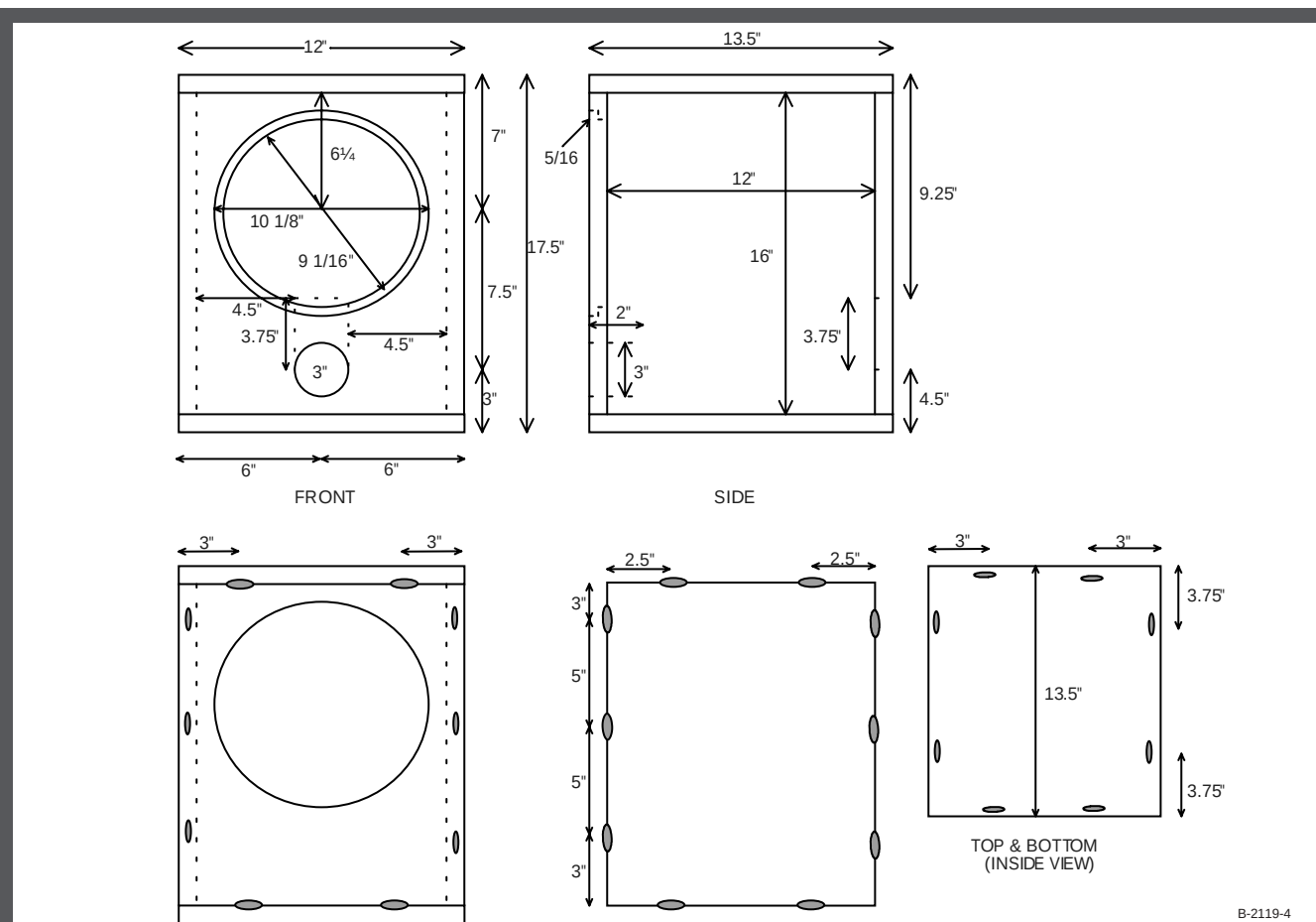
FIGURE 4: Diagram of box, including biscuit placement.
