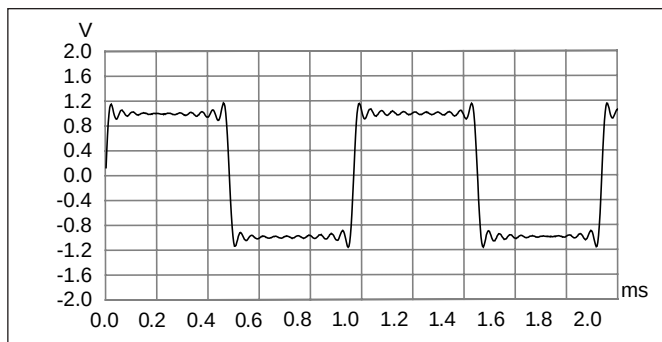
FIGURE 9: 1kHz square-wave response.
