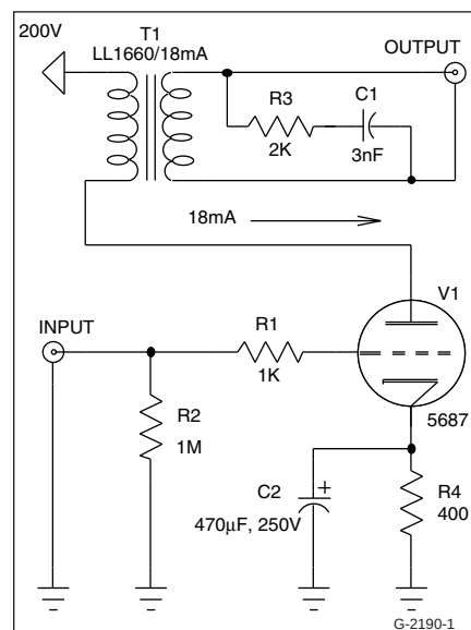
FIGURE 1: Single-ended line stage. Lundahl provided this design, using the LL1660/18mA transformer.
