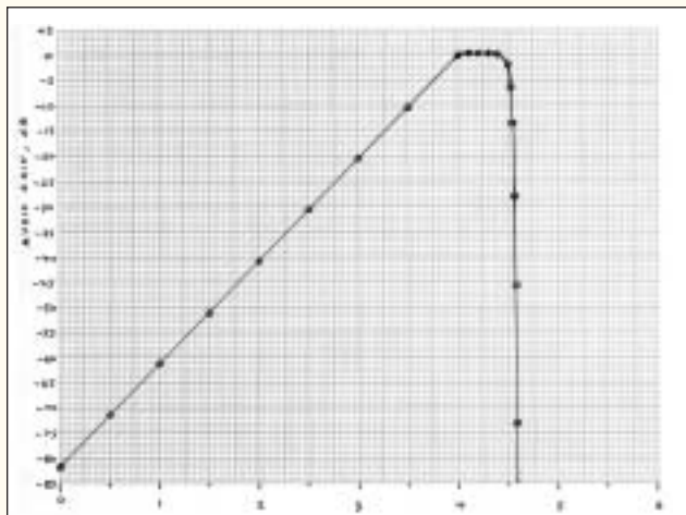
FIGURE 3: Remote control input vs. audio gain.
