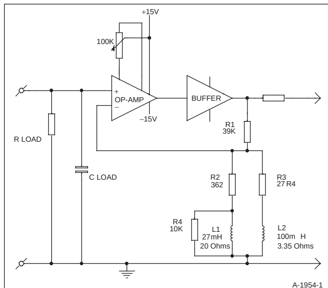
FIGURE 1: Example op-amp/ inductor RIAA stage, after M. Danbury.
