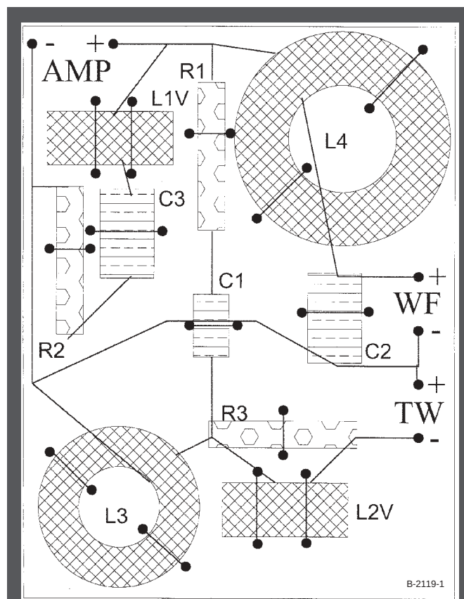
FIGURE 1: Suggested layout (from Adire Audio assembly instructions).
