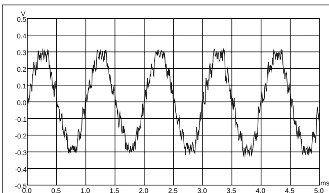
FIGURE 9: Undithered 1kHz sine wave at -90.31 dBFS.
