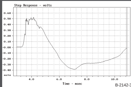
FIGURE 3: Adire step response.
