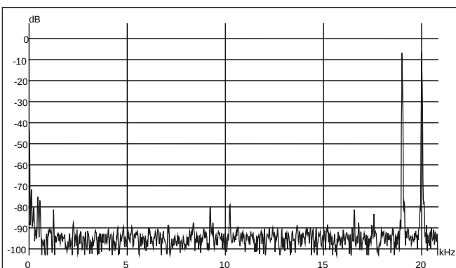
FIGURE 8: Intermodulation distortion, 19 + 20kHz 0dBfs (OPA604).
