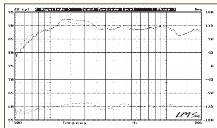
FIGURE 11: SPL of tweeter on enclosure with 2" radius shell versus enclosure without edge treatment (solid line); difference curve raised 60dB.
