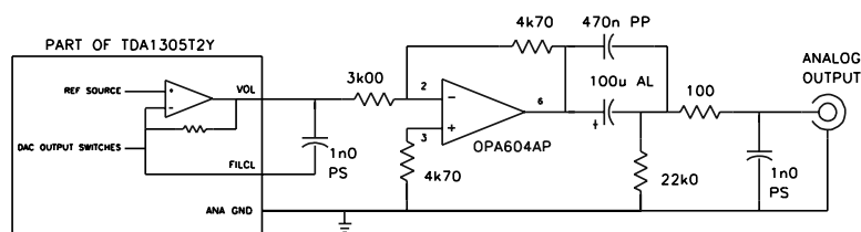
FIGURE 2: Modified analog output stage.
