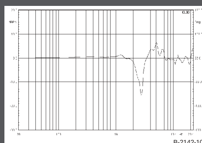
FIGURE 10: HE10.1 response difference (#2 minus #1).
