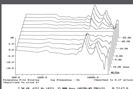
FIGURE 8: Adire vertical polar response.
