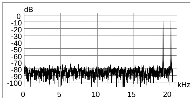
FIGURE 8: Spectrum of 19kHz + 20kHz intermodulation signal.
