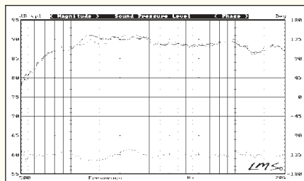
FIGURE 2: SPL of tweeter on IEC baffle with midbass covered (solid line) versus with midbass uncovered; difference curve shows diffraction from midbass cavity.
