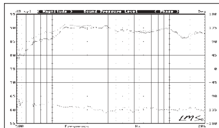
FIGURE 17: SPL of tweeter on enclosure with dual beveled shell versus on IEC baffle (solid, lower line); difference curve raised 60dB.
