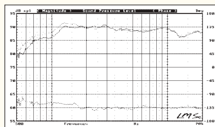
FIGURE 6: SPL of tweeter on enclosure with 4" radius shell versus on IEC baffle (solid, lower line); difference curve raised 60dB.
