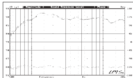
FIGURE 19: SPL of tweeter on enclosure with 4" beveled shell versus enclosure without edge treatment (solid line); difference curve raised 60dB.
