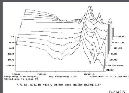
FIGURE 5: Adire horizontal polar response.
