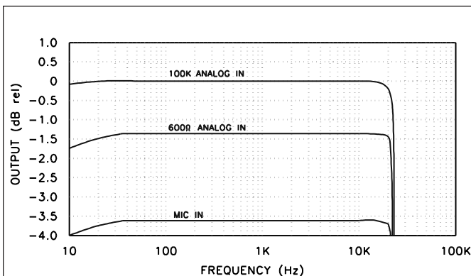
FIGURE 1: Frequency response.
