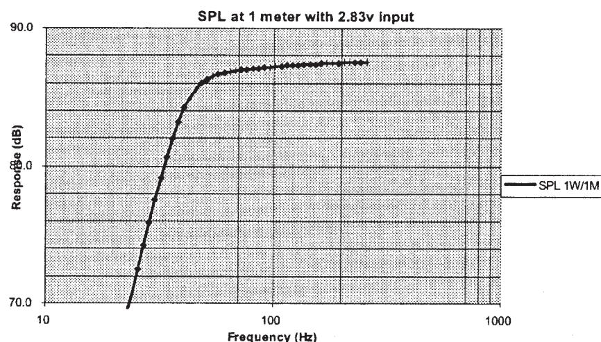
FIGURE 5: Maximum bass extension alignment for vented boxes per Weems, driver Q_{TS} = 0.3 , f_s = 30 , V_{AS} = 50 ltr.
