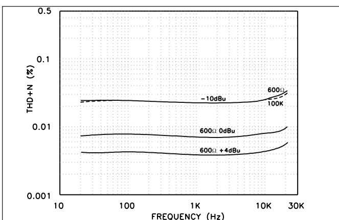
FIGURE 2: THD+N versus frequency.
