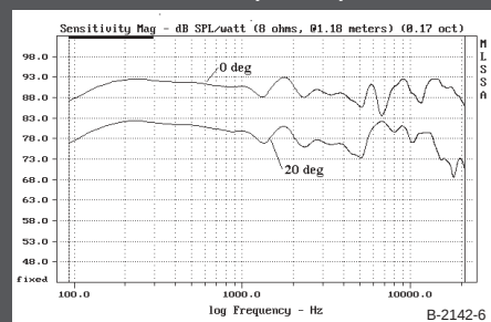
FIGURE 6: Response at 0 and 20° horizontal (20° offset -10dB).
