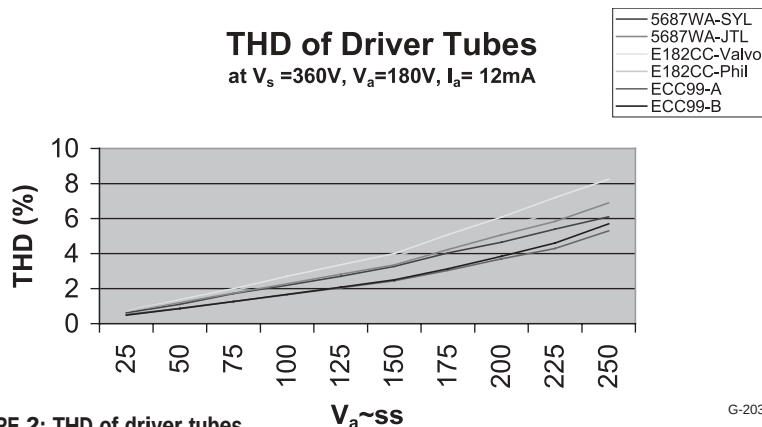
FIGURE 2: THD of driver tubes.
