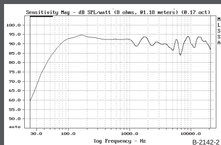
FIGURE 2: Adire full-range frequency response.
