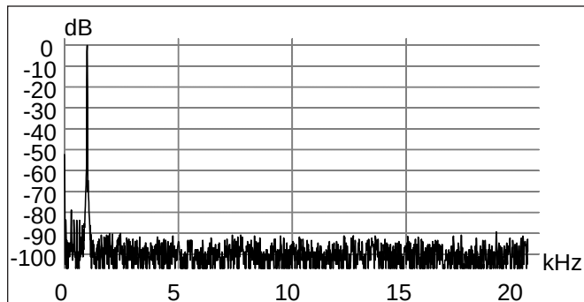
FIGURE 7: Spectrum of 1kHz sine wave.
