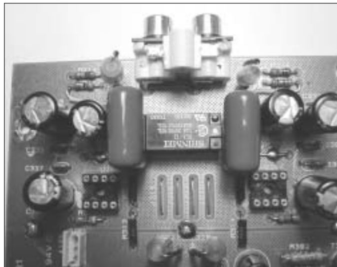
PHOTO 4: Detail of MPP capacitor installation.
