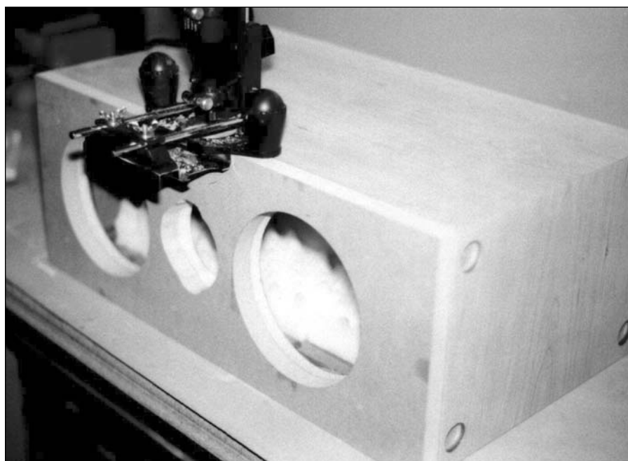
PHOTO 15: Cutting the reveal groove with Dremel tool on router base. Note: veneer is applied at this point.
