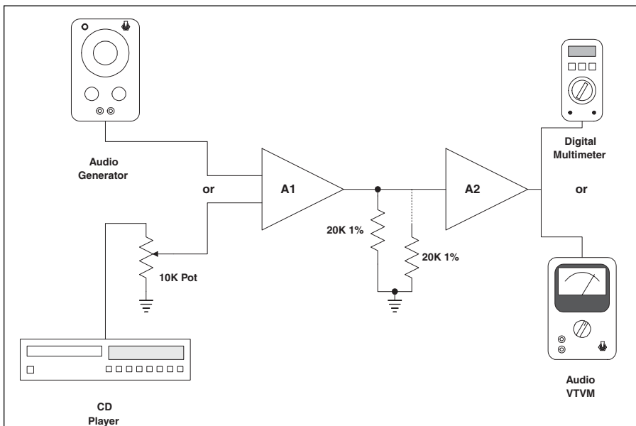
FIGURE 6: Setup for measuring output impedance of A1. The dashed line denotes a clip-lead that is removed during the test.
