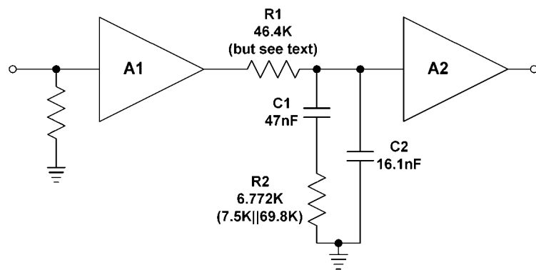
FIGURE 2: Passively equalized phono preamp circuit; with the values shown, this yields the RIAA curve. For typical moving-magnet cartridges, the two amplifiers should have a total gain of about 60dB. See text for discussion of R1's value.
