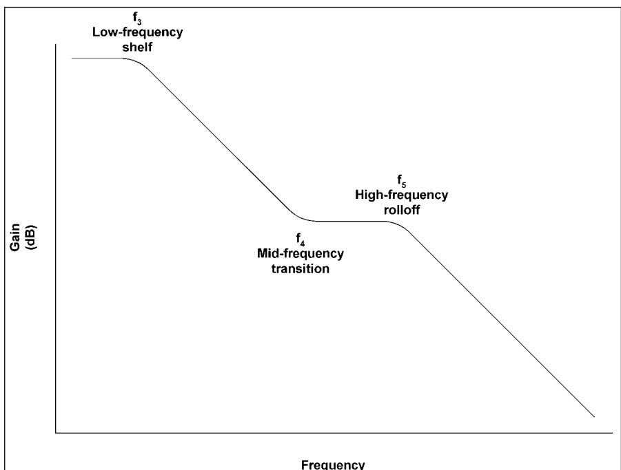
FIGURE 3: Generalized phono equalization curve.
