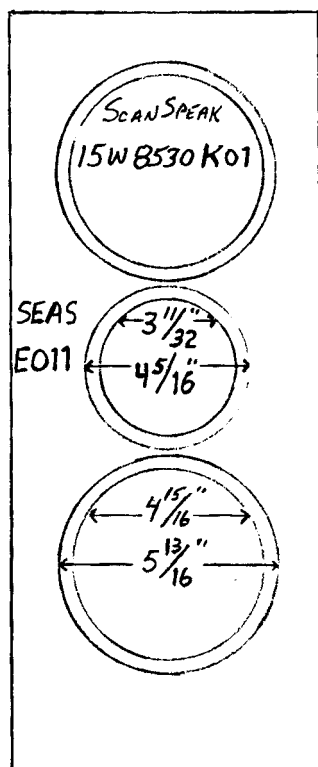
FIGURE 10: Satellite driver cut-out diagram.
