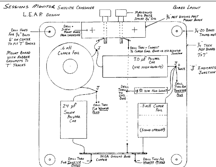
FIGURE 11: Satellite crossover physical layout.
