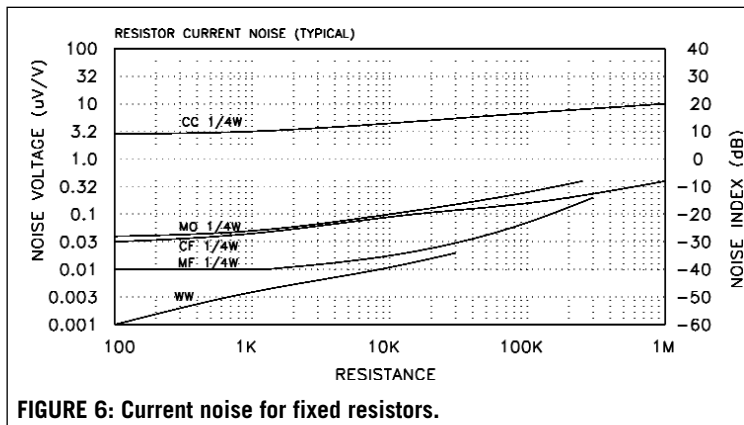
FIGURE 6: Current noise for fixed resistors.
