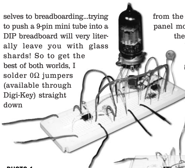
PHOTO 1: Breadboarding a tube.
