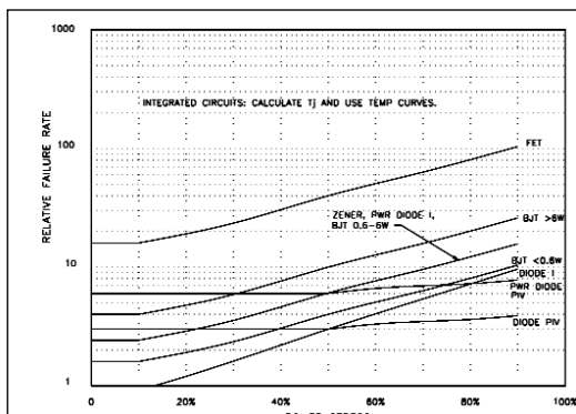
FIGURE 9: Semiconductor failure rates versus electrical stress.
