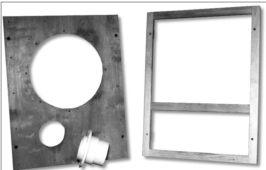
PHOTO 3: Low-frequency enclosure baffle and grille frame.
