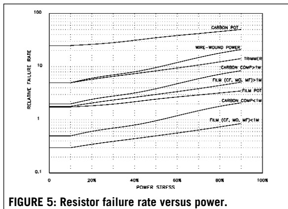
FIGURE 5: Resistor failure rate versus power.
