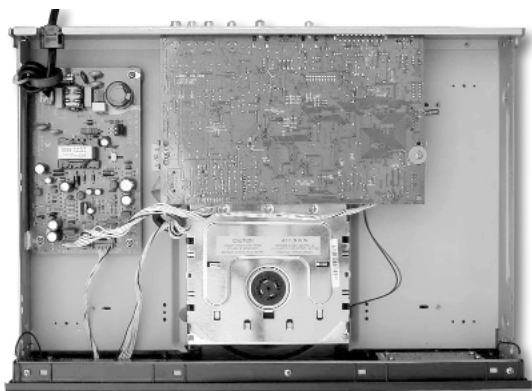
PHOTO 3: Inside the T550. The main PC board is mounted upside down. The switching power-supply board is on the left.
