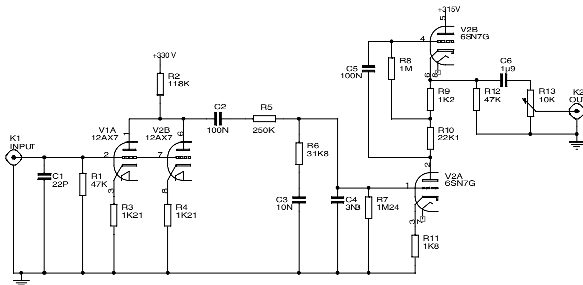
FIGURE 1: Phono preamp circuit.
