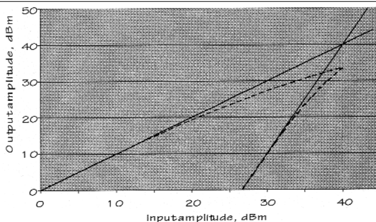
FIGURE 8: Amplitude response of amplifier displaying "classical" third-order IMD. Amplifier input signal level is displayed on the X-axis, and output level on the Y-axis; both axes are logarithmic. The straight line through the origin represents ideal linear response. The straight line at a steeper angle shows the theoretical level of IMD products, which change three times as quickly with input amplitude as the signal itself. The point where the straight lines meet is the IP3. The curved lines show the likely real characteristics as the amplifier begins to clip. However, for sensible operating points well below the IP3, the straight lines are a fairly good match for a single-stage class-A RF amplifier without any special linearization techniques. The IP3 concept is also useful for other devices such as mixers, which also display IMD. For any input signal level on the X-axis, the upper line will show the nominal output level, and the vertical separation between the two straight lines will show the expected linearity in dBc. When high-level multi-tone signals are concerned, this figure—rather than the noise figure—usually represents the dynamic range of the signal, since it indicates the relative level of interfering products.
