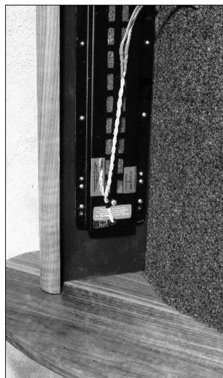
PHOTO 29: Positioning the driver.
