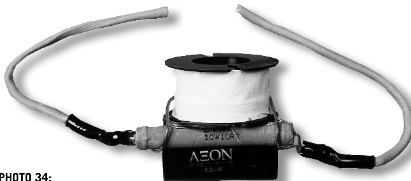
PHOTO 34: Factory passive filter.
