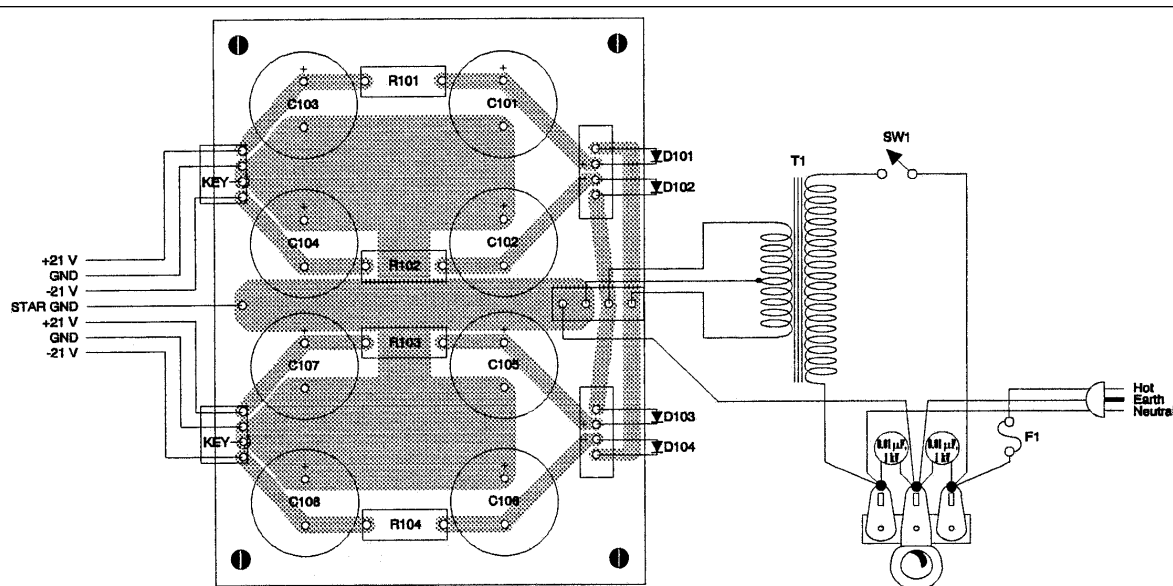
Figure 6: Power-supply-enclosure construction pictorial.
