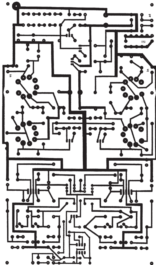
◀ FIGURE 8: Power-stage board.
