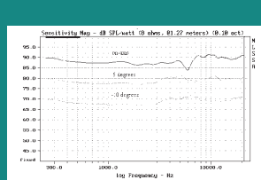
FIGURE 10: Vertical response at 0, -5^\circ , and -10^\circ .
