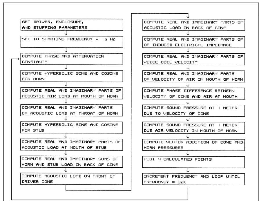
FIGURE 8: Simulation-program flowchart.
