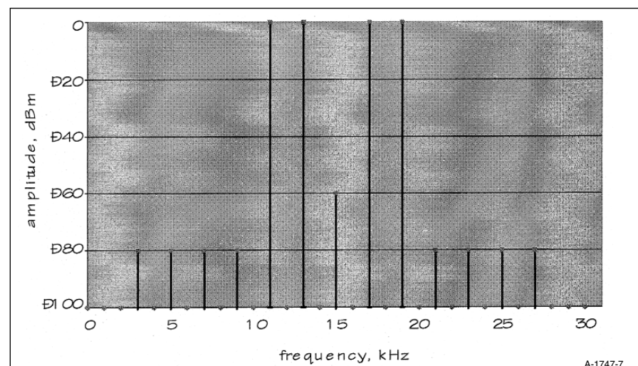
FIGURE 7: Idealized spectrum of four-tone test sometimes used with RF amplifiers. The four main tones are harmonically related, phase-locked and phase-peaked to maximize the peak value of the signal envelope in the time domain. This—in an RF amplifier, at least—is likely to maximize the visible third-order IMD products, particularly the central one between the two pairs of tones which thus makes an easy frequency component to check. With zero IMD this component would be completely absent.
