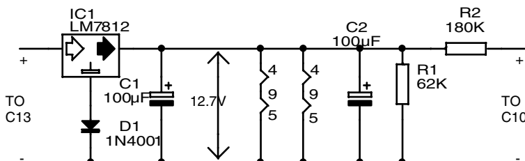
FIGURE 3: Stabilization section.
