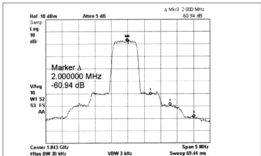
FIGURE 10: Example of a real modulated signal with IMD—here the IMD products are not discernible individually but serve effectively to raise the noise level in steps—each step corresponds to a particular order of IMD. The first step on each side is produced by third-order IMD, the next by 5th, the next by 7th, and so on. Note that the IMD products occupy more bandwidth than the original signals; the higher the order, the more bandwidth occupied. The step pattern might, however, not be visible with the less-ordered spectrum of a typical music signal.
