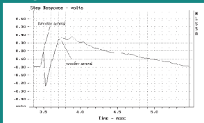
FIGURE 5: Step response.
