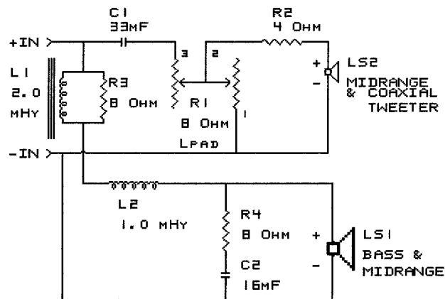
FIGURE 3: Speaker-system electrical schematic.
