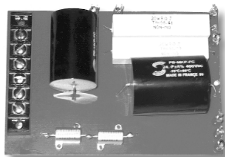
PHOTO 2: Component side of crossover board showing resistors, capacitors, and posts for connections to external components. (The series-connected resistors are a substitute for the specific parts, which were out of stock.)
