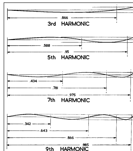
FIGURE 17: This chart is to aid in identifying the various odd-order harmonics present from the shape of the transfer characteristic. The fractions give the points at which the curve should cross the straight fundamental line, when only that harmonic is present in the signal.
