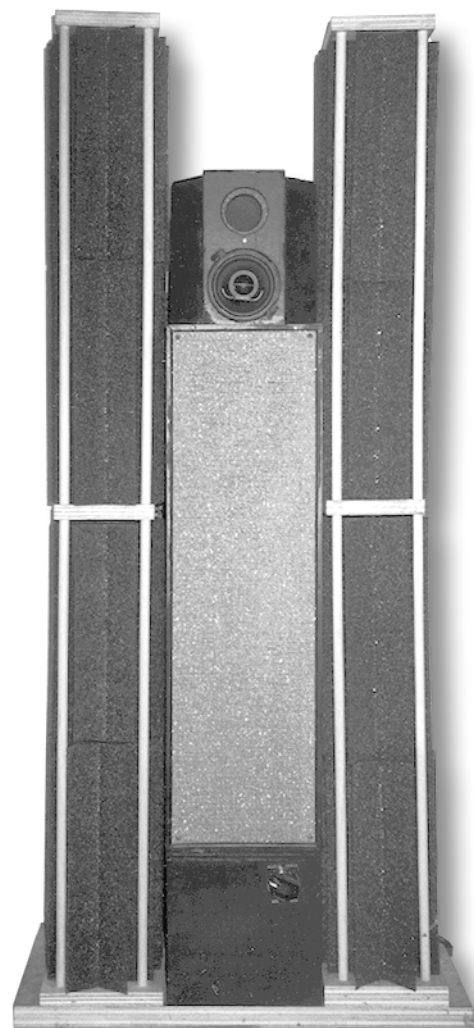
PHOTO 1: The revised left channel complete with absorbers. The treble unit is placed vertically and is flanked by 1.75"-thick blocks with 45° ends.
