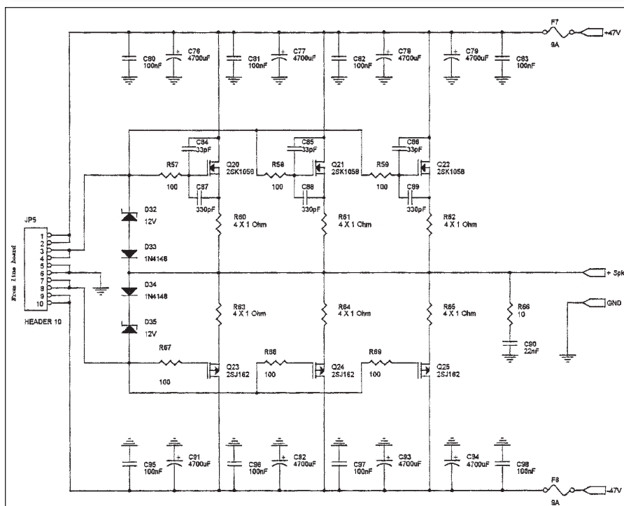
FIGURE 4: 150W power-board schematic.
