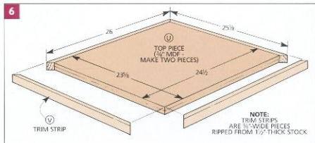
A built-up top with a large opening allows sawdust to fall into the dust bin below. It also provides a sturdy platform for mounting the table saw.
