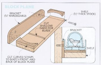
Curved scraps of hardboard keep a block plane from falling off a thin wood shelf. Gluing a bracket to the shelf makes the holder easy to mount.
