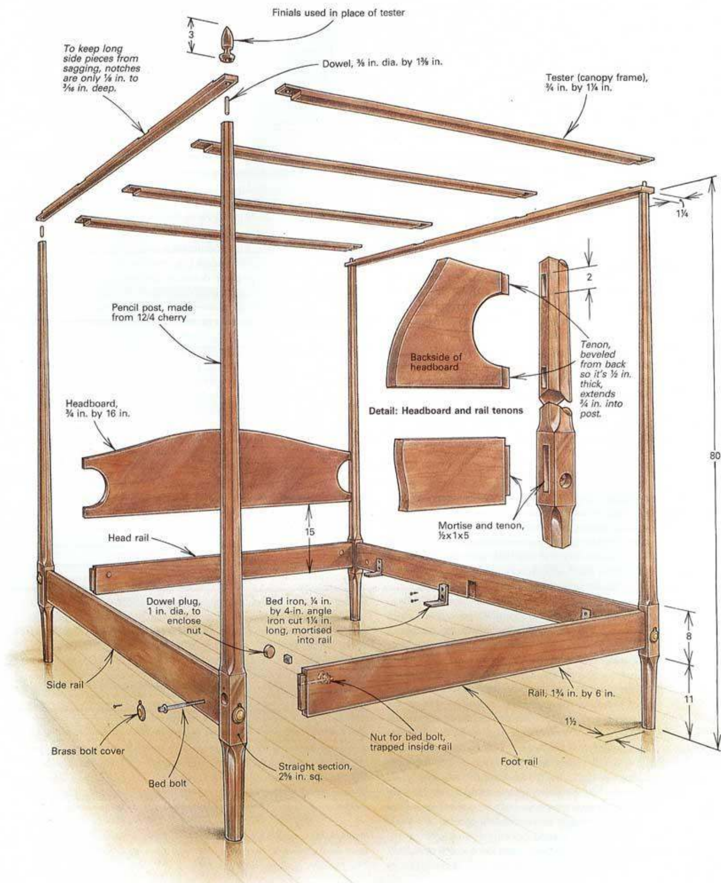
Fig. 1: Pencil-post bed
