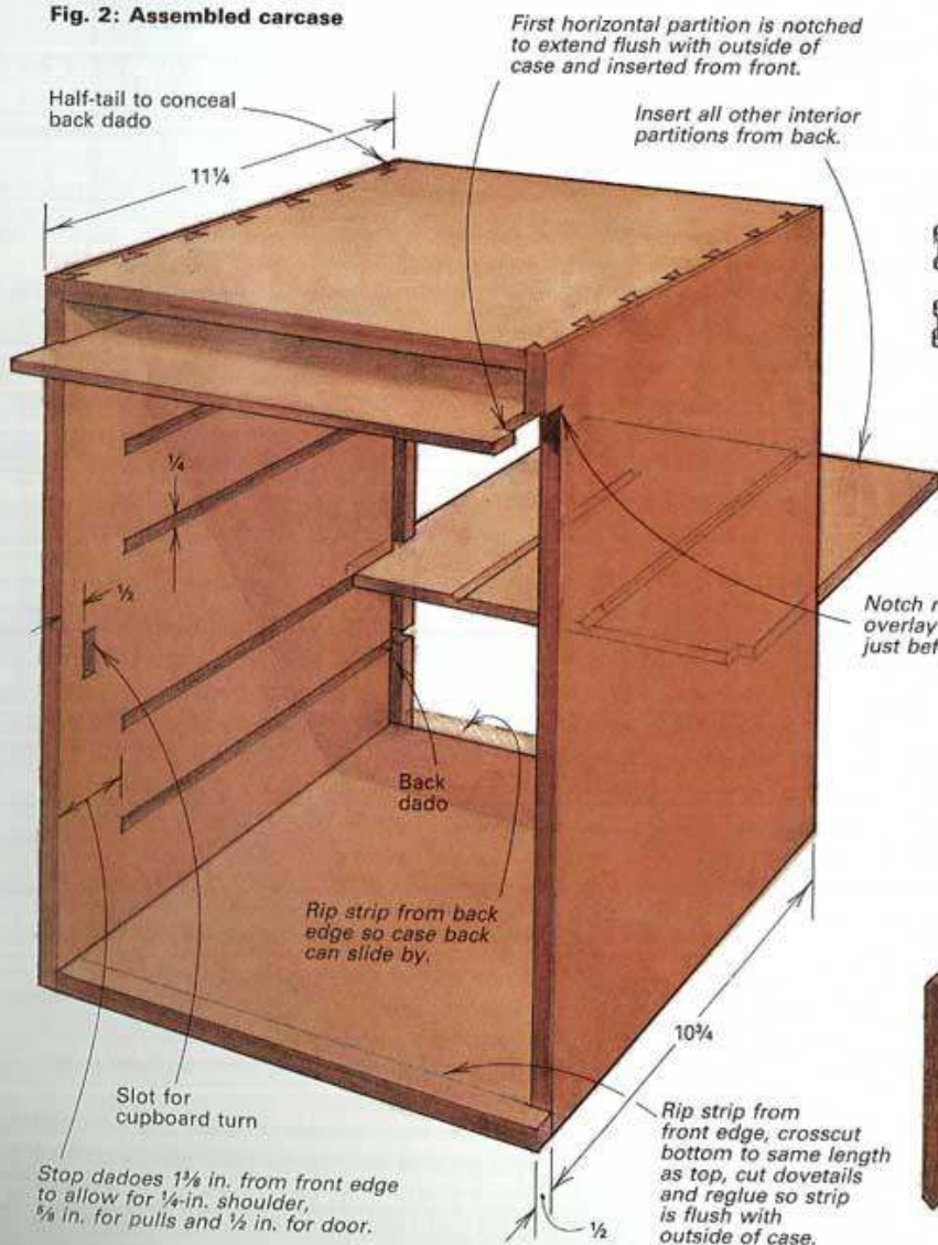
Fig. 2: Assembled carcass
