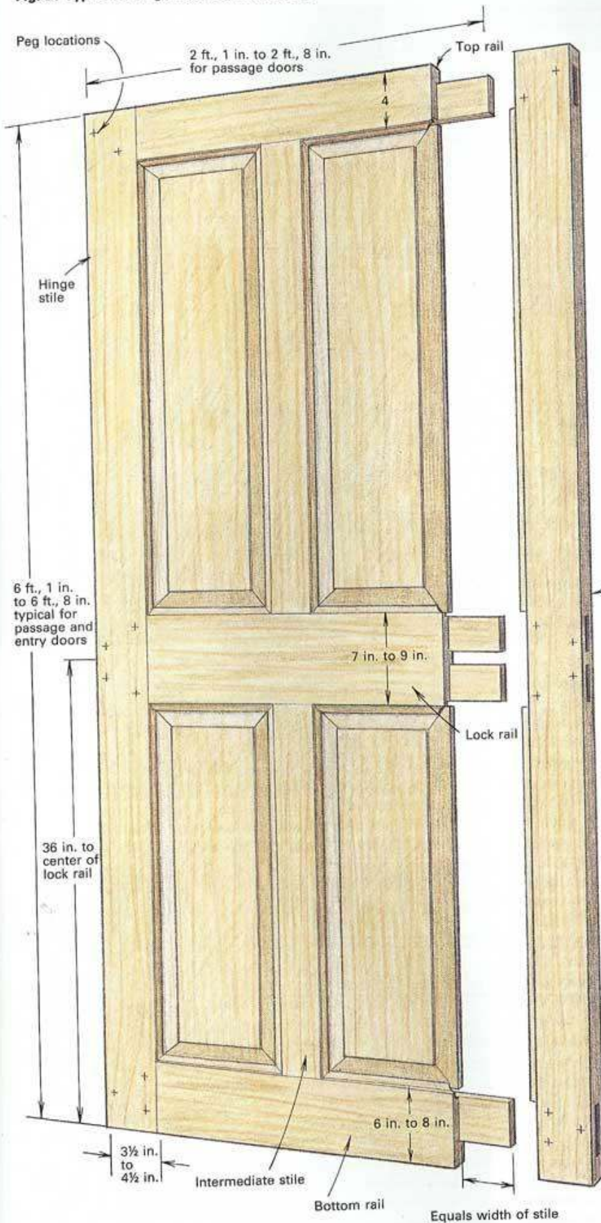
Fig. 2: Typical Georgian-period panel door
