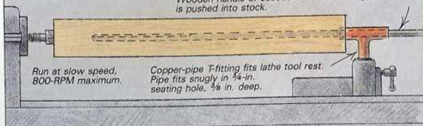
Fig. 1: Boring the housing
