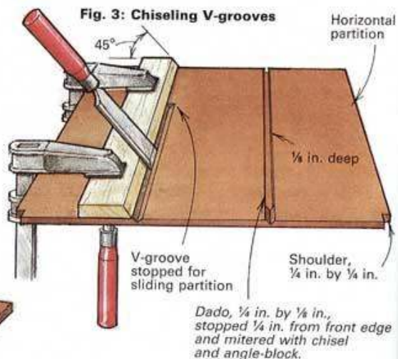
Fig. 3: Chiseling V-grooves
