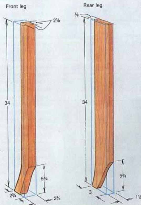
Fig. 2: Leg construction
