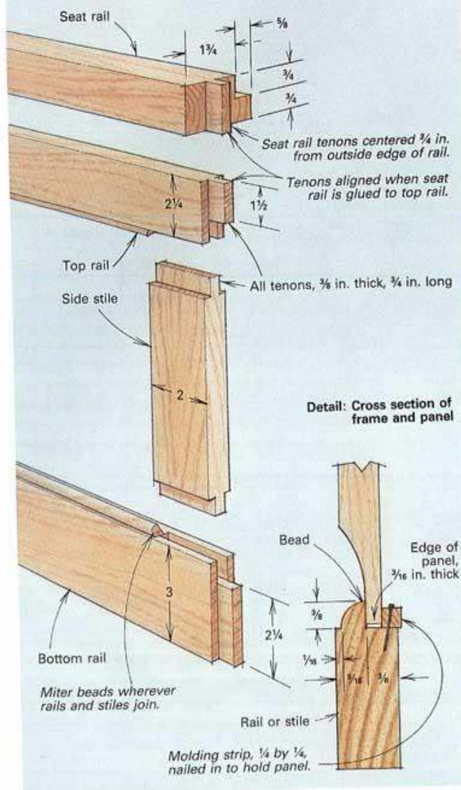
Fig. 3: Frame-and-panel construction
