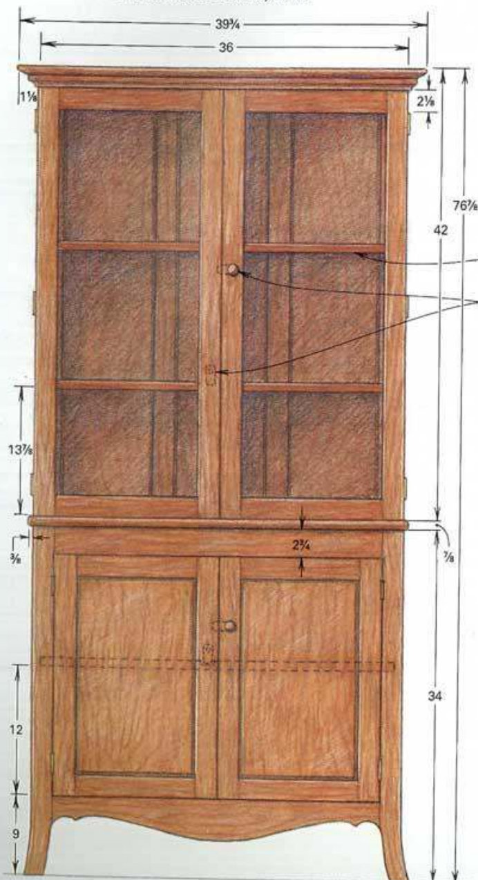
Fig. 1: Cupboard plans
