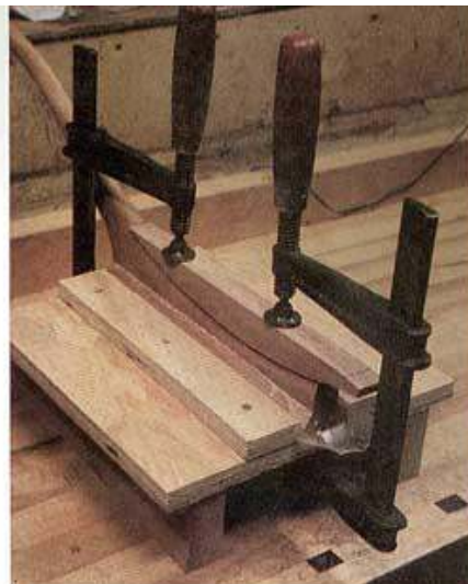
These three photos show the fixture and clamping arrangements used for assembling two legs with a filler block (left); two filler blocks with a leg (center); and the final pedestal glue-up (right). A scrap piece, left over from the bandsawing of the legs, is used as a caul.
