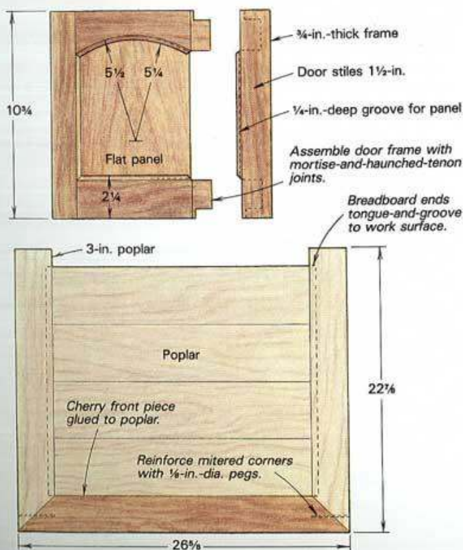
Fig. 2: Writing slide and cupboard door
