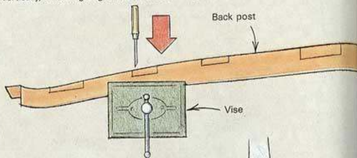
Fig. 7: Crest-rail mortises
