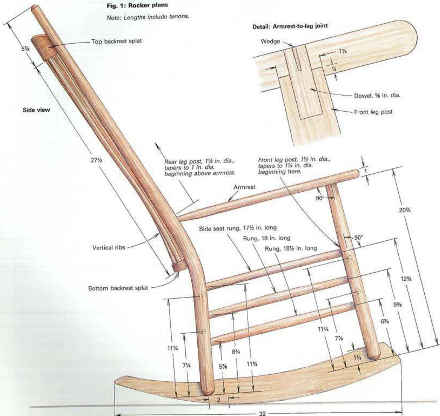
Fig. 1: Rocker plans
