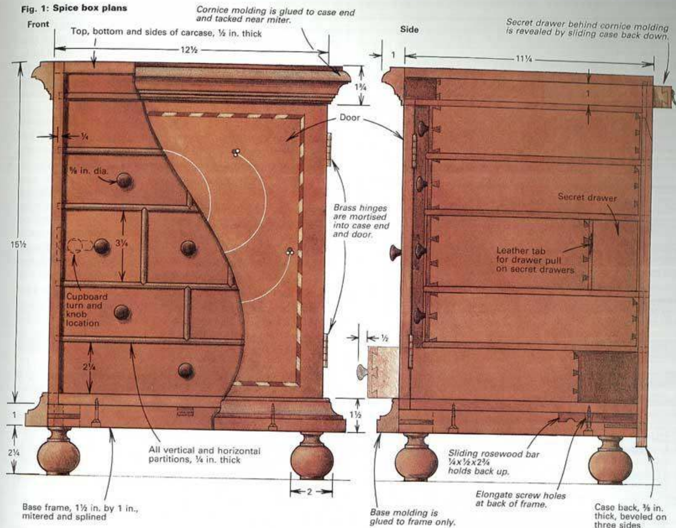
Fig. 1: Spice box plans
