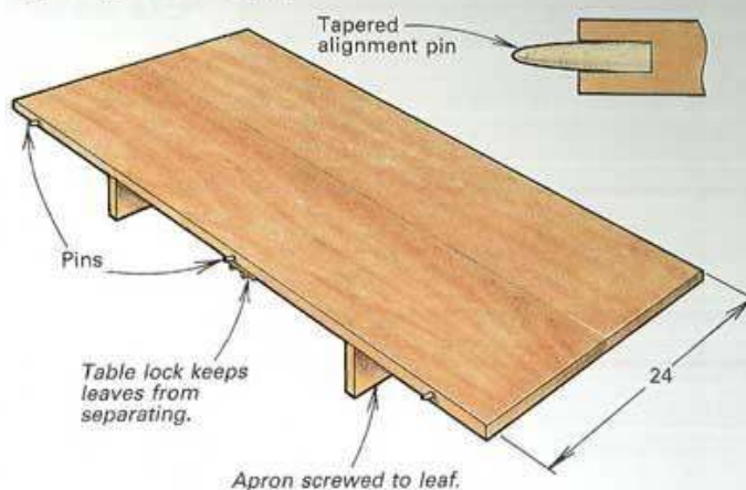
Fig. 3: Typical leaf detail
