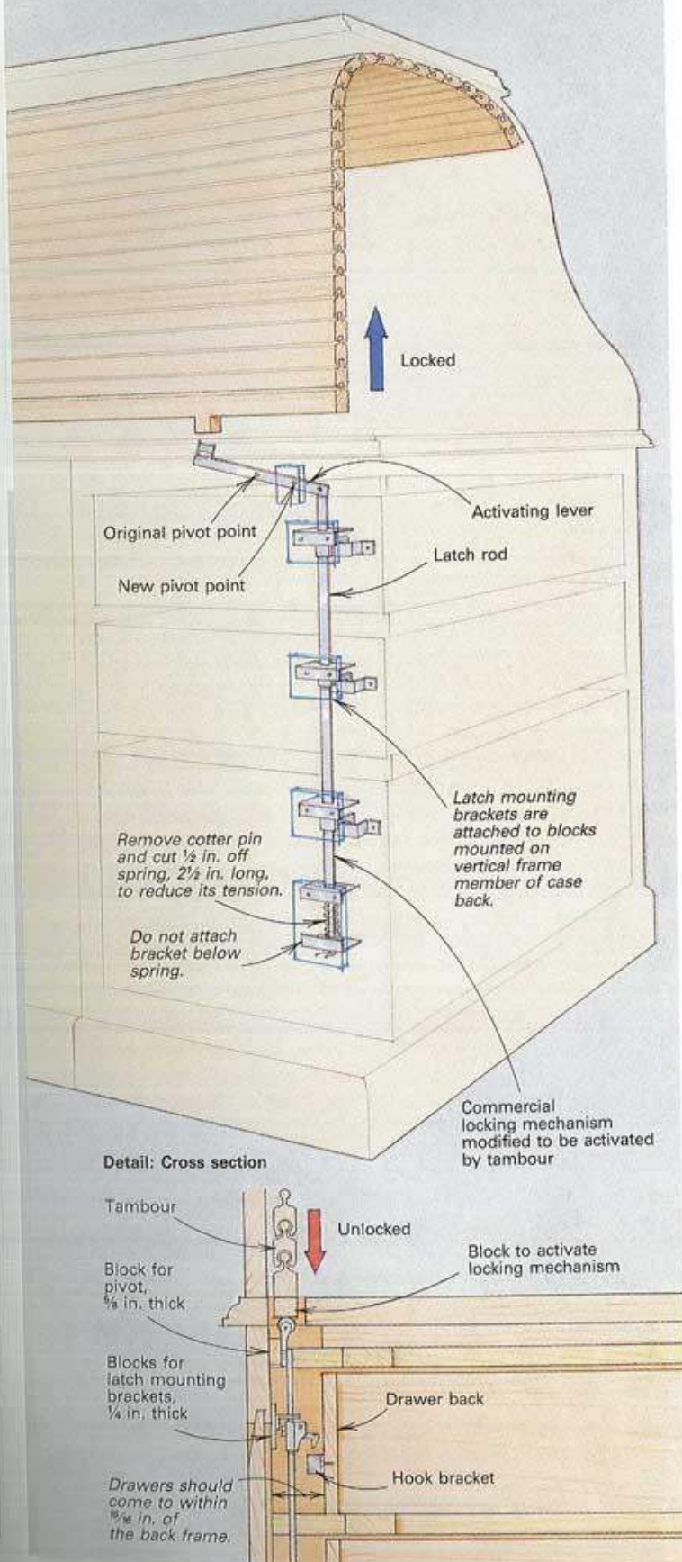
Fig. 4: Locking mechanism
