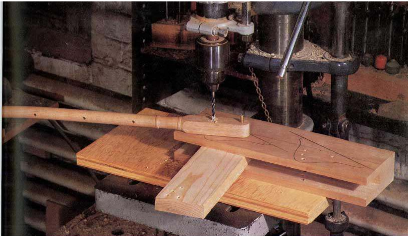
To ensure that the stem and hinge are properly aligned, use the \frac{1}{8} -in.-dia. hole bored in the stem as a guide for drilling the hinge blank. A screw or pin inserted through the hinge and the stem holds the pieces together while the holes are bored.
