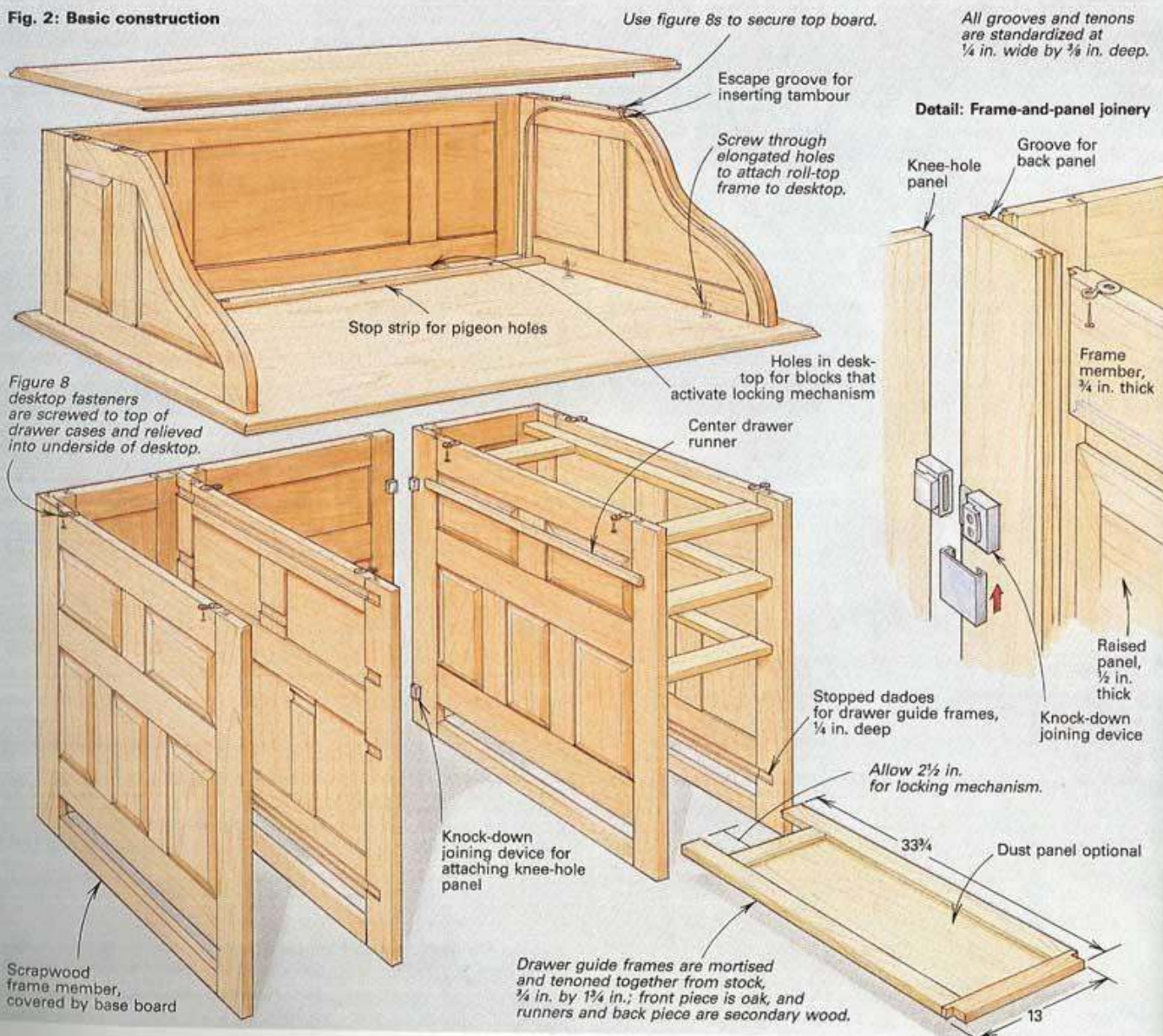
Fig. 2: Basic construction
