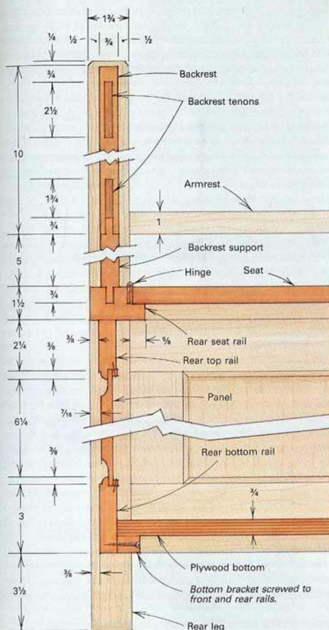
Fig. 2: Cross section through rear of Sengebenk
