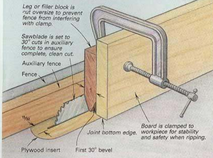
Fig. 4: Tablesaw setup for bevel cuts
