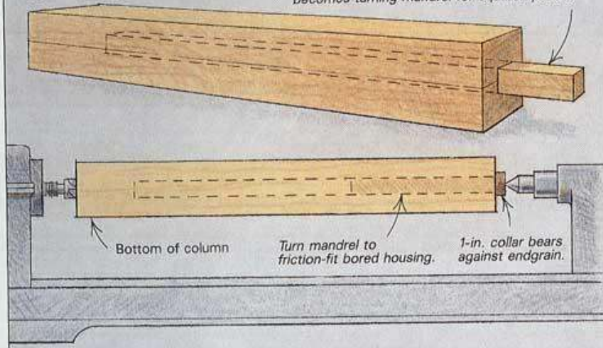
Fig. 3: Turning hollow spindles
