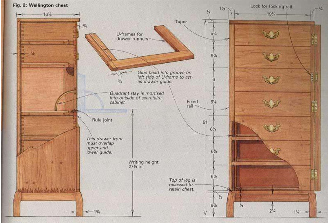
Fig. 2: Wellington chest
