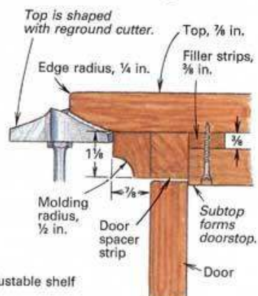
1A: Top corner molding detail
