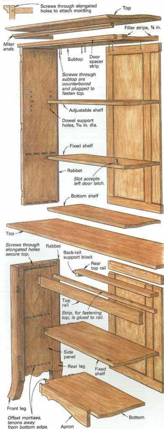
Fig. 3: Cupboard construction
