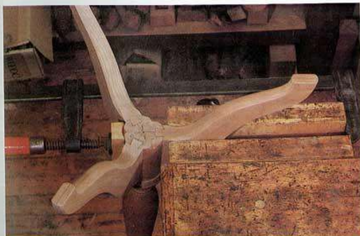
If necessary, you can secure one leg in a bench vise and use a clamp as shown to pull the shoulders tight on the tails.
