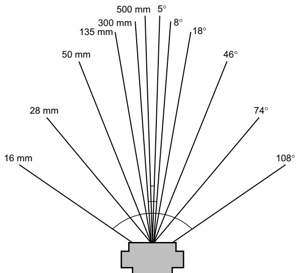
Figure 5.2 Angles of view given by lenses of different focal lengths used on a 35 mm format camera. Left: The same view photographed using different focal length lenses without changing the camera position
