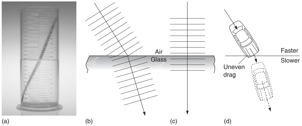
Figure 2.10 Refraction. Light slows when passing from air into glass. Wavefronts slow unevenly if light reaches the denser medium obliquely (b). The effect is like driving at an angle from the highway onto sand (d). Uneven drag causes change of direction. Light striking the boundary at right angles (c) slows but does not alter direction
