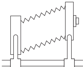
Figure 4.19 Rising front. A view camera offering this camera movement is still often used for architectural subjects where most elements are well above the lens centre. Tilting a normal camera upwards would make vertical lines converge. Instead, the camera back here was kept upright and the front lens standard raised to include more arch top, less road (see also digital manipulation of perspective, p. 367)
