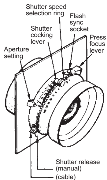
Figure 4.12 Shutter and lens unit. Typical view camera ( 5 \times 4 ) lens unit with mechanical bladed shutter. The panel it is mounted on makes it interchangeable with other lens units
