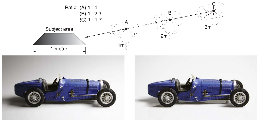
Figure 7.7 Distance and evenness. Left: A hard light source positioned obliquely at A is too close to the subject – the nearest part of this model car receives four times more light than the farthest end. Right: Pulled back to position C, three times the original distance, this ratio is reduced to 1.7 times. The subject is much more evenly lit and easier to expose correctly
