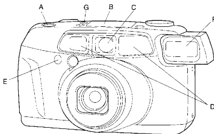
Figure 4.21 A typical direct viewfinder compact camera. (A) Shutter release and power wind-on. (B) LCD panel, displaying frame counter, battery state, etc. (C) Front window of viewfinder. (D) Windows for IR auto-focus system. (E) Light sensor for auto-exposure setting program. (F) Flip up or pull out flash. (G) Lens zooming control
