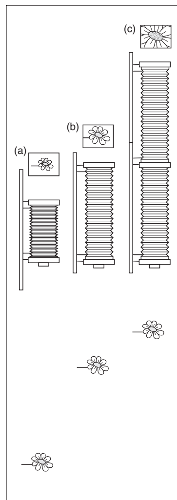
Figure 5.17 Bellows extension needed for close-ups. (a) View camera focused on distant subject. (b) Imaging the subject life size requires bellows twice the lens focal length. (c) The same lens needs two sets of these bellows and an extension rail, to image the subject three times life size. See also Figure 2.20
