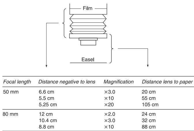
Figure 12.8 The ‘throws’ necessary for a 35 mm enlarger (50 mm lens) and 120 film enlarger (80 mm) to achieve various image magnifications. Most 35 mm standard column enlargers allow the lens to be raised at least 60–70 cm above baseboard
