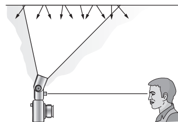
Figure 10.36 'Bouncing' flash. The light sensor must continue to face the subject direct. Illuminate the ceiling above the camera, not subject – otherwise you risk shadowed eyes
