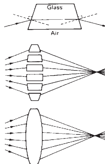
Figure 2.16 Lens evolution. Top: Using a non-parallel sided glass block (prism), refraction at each air/glass surface (compare with centre of Figure 2.9) causes an overall change of direction. Think of a lens shape as a series of blocks which bend many light rays to a common point of focus
