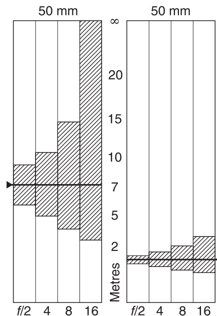
Figure 3.11 Depth of field at different apertures when a 50 mm lens is focused for 7 m (left) and for 1.5 m (right). The symbol denotes infinity. Depth of field is greatly reduced with close subjects
