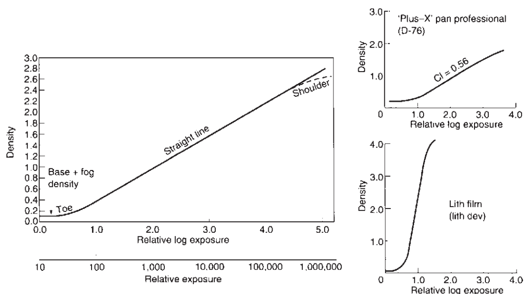
Figure C.3 Characteristic curves of various monochrome films
