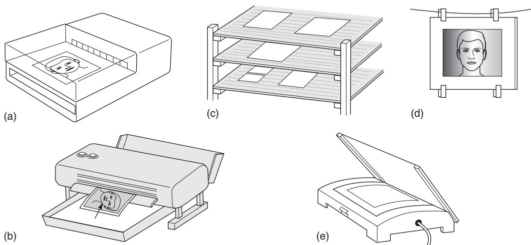
Figure 12.30 Print drying. (a) Fan-assisted warm air dryer, for up to two RC prints at a time. (b) Fast, hot-air dryer for RC paper only; print must be inserted covered by a film of water, direct from tray. (c) Ambient air drying, using fine mesh racks or (d) line pegging. (e) Flat bed heated dryer, with glazing sheet for fibre base glossy paper
