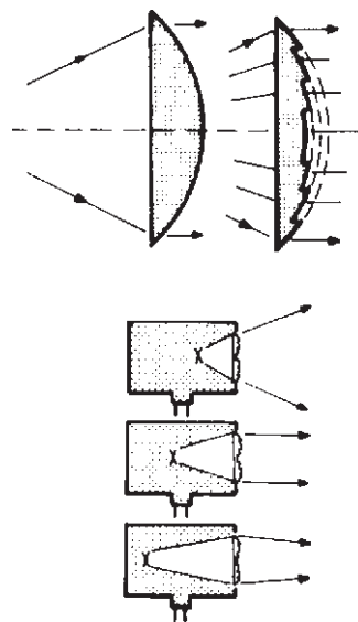
Figure 7.11 Focusing spotlight. Top: Shaped 'Fresnel lens' bends illumination like the fatter lens (left) but is less bulky, with larger cooling surface. Bottom: Shifting the lamp position in a focusing spotlight adjusts the beam width. Broadest beam gives hardest, most point-like lighting; see also Figure 2.5
