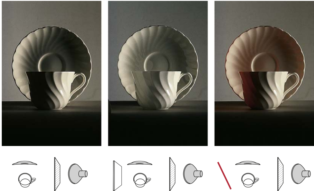
Figure 7.6 Controlling lighting contrast. All three pictures are lit by one diffused floodlight about 90° from one side. Left: No fill-in. Centre: A large matt white reflector is added left, directly facing the light. Right: Using red instead of white reflector board
