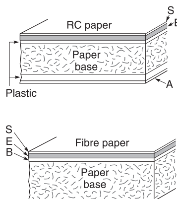
Figure 12.16 Cross-sections of RC and (single weight) fibre bromide papers. S: Supercoat of clear gelatin. E: Emulsion. B: Whitening baryta coating. A: Anti-static layer
