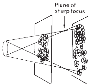
Figure 2.17 A converging lens bends diverging beams of light to a point of focus. However, if the lens-to-screen distance is incorrect, either too near or too far as shown right, images again consist of fuzzy 'circles of confusion'. (This is why out of focus highlights become discs – Figure 2.18)
