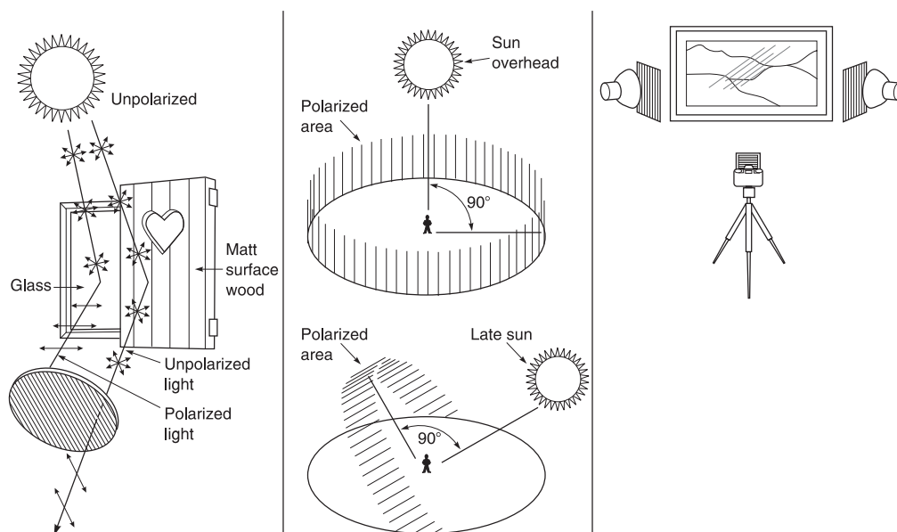
Figure 9.32 Using a polarizing filter. Left: To absorb light reflected from a glass window – most strongly polarized at 33^\circ to the surface. Light scattered from the matt-surfaced wood remains unpolarized, and passes through the camera filter. Centre: Rotating the polarizing filter darkens parts of blue sky at right angles to the sun's direction. Right: All reflections removed from glass by polarizing the light from the lamps and fitting another filter (turned 90^\circ ) over the camera lens
