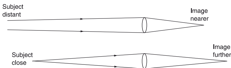
Figure 2.21 The closer the subject to a lens, the greater the distance it needs to bring the light into sharp focus. Light rays from a distant subject point are more parallel, so the same lens bending power brings them to focus nearer to the lens
