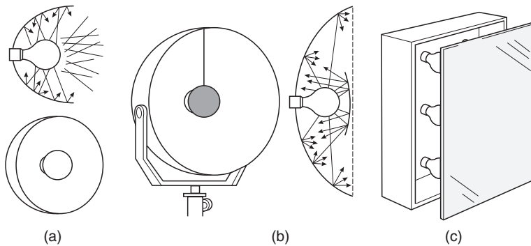
Figure 7.12 Tungsten lamp units for soft illumination. The larger the unit the more diffused the light. They use 3200 K diffuse-glass floodlamps in (a) matt white open-fronted reflector, (b) wider dish flood with direct light shield and (c) large opal plastic-fronted box giving lighting quality similar to overcast light from a window
