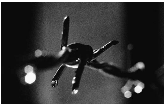
Figure 2.18 This image was made with a wide-diameter lens focused for one droplet on the barbed wire. Droplets closer (left) and farther away (right) become unsharp patches of light at this focus setting. Notice how each patch takes on the shape of the lens diaphragm
