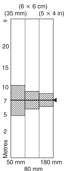
Figure 3.17 Depth of field when standard focal length lenses for different formats are used at an identical aperture ( f/4 here). All were focused for 7 m. Larger format cameras produce less depth of field because they use longer focal length lenses
