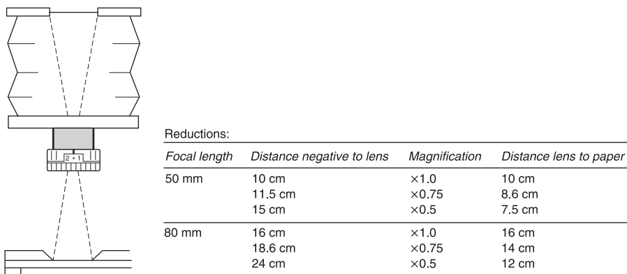
Figure 12.9 Enlargers may also allow you to make reduced size prints, provided the lens will move far enough from the negative. If bellows are too short add a camera extension tube. Check that the image remains evenly illuminated
