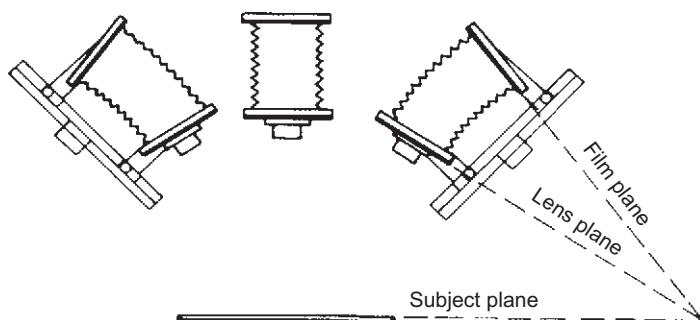
Figure B.8 The Scheimpflug correction, to maximize depth of field over a subject plane imaged obliquely. Note how the subject, lens and film planes all meet at one point. This uses some swing of both front and back, minimizing the side effects of each movement (see Figure B.9). Note that when all three planes are parallel as in the centre position the lines meet theoretically at infinity
